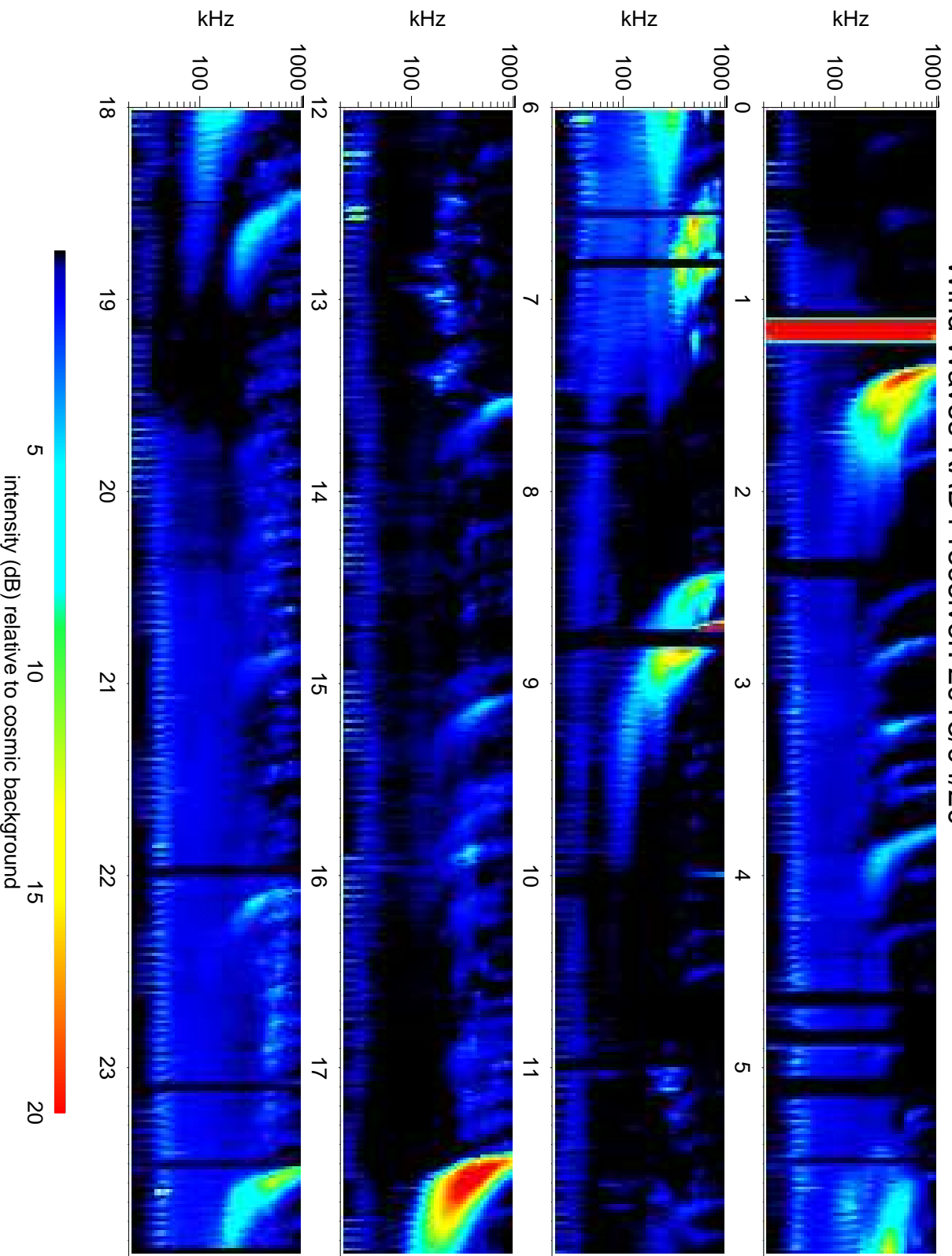
Wind Waves RAD1 receiver: 2013/04/20
