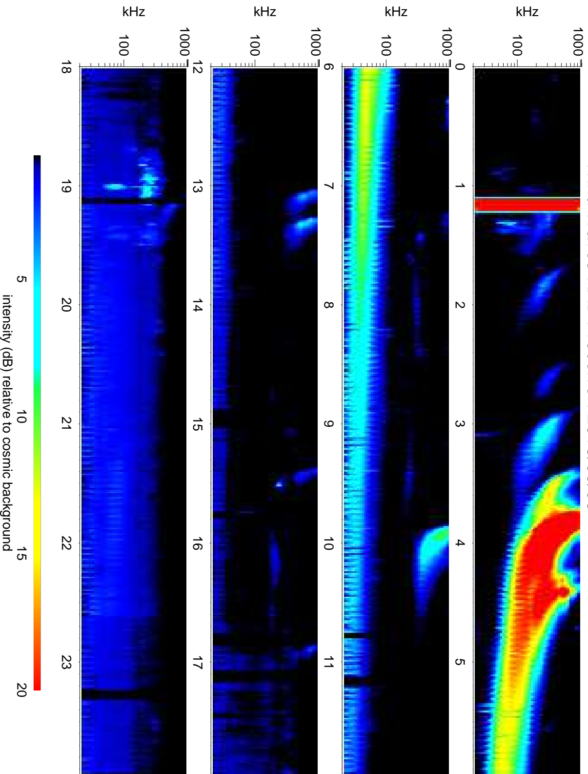
Wind Waves RAD1 receiver: 2013/03/05
