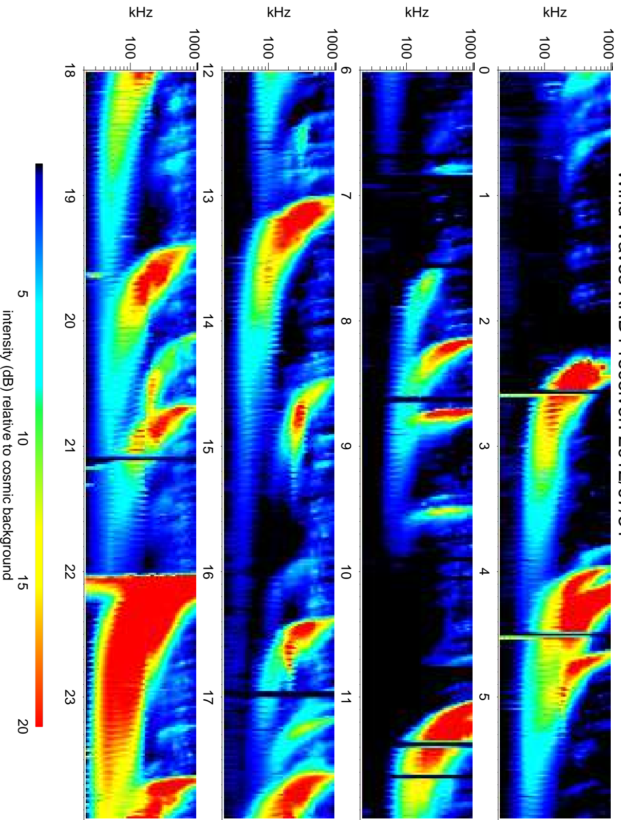
Wind Waves RAD1 receiver: 2012/07/31
