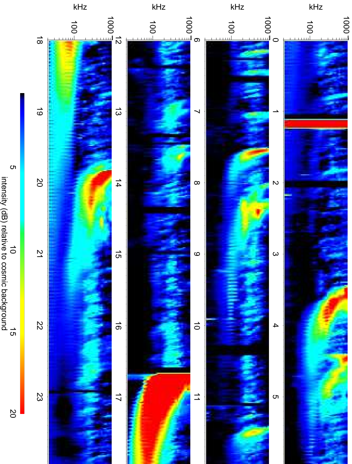
Wind Waves RAD1 receiver: 2012/07/04
