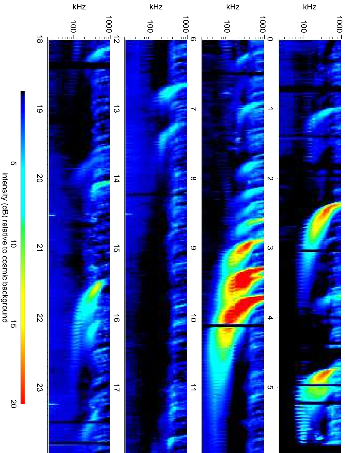
Wind Waves RAD1 receiver: 2012/05/14
