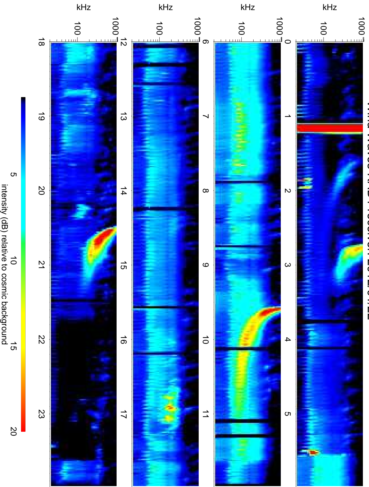
Wind Waves RAD1 receiver: 2012/01/22
