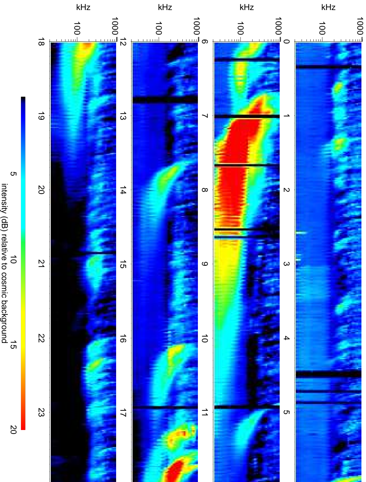
Wind Waves RAD1 receiver: 2011/1/11/1
