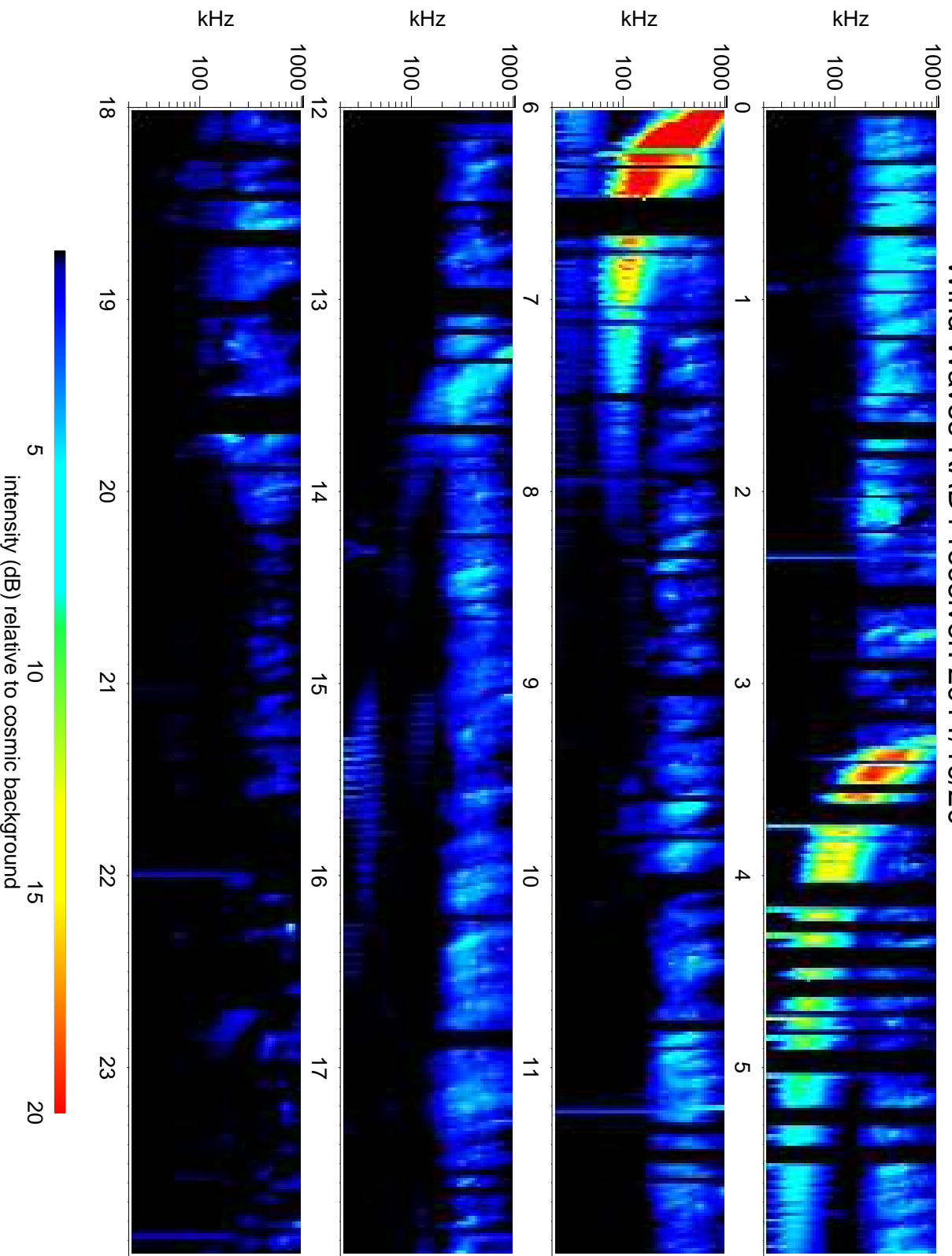
Wind Waves RAD1 receiver: 2011/10/20
