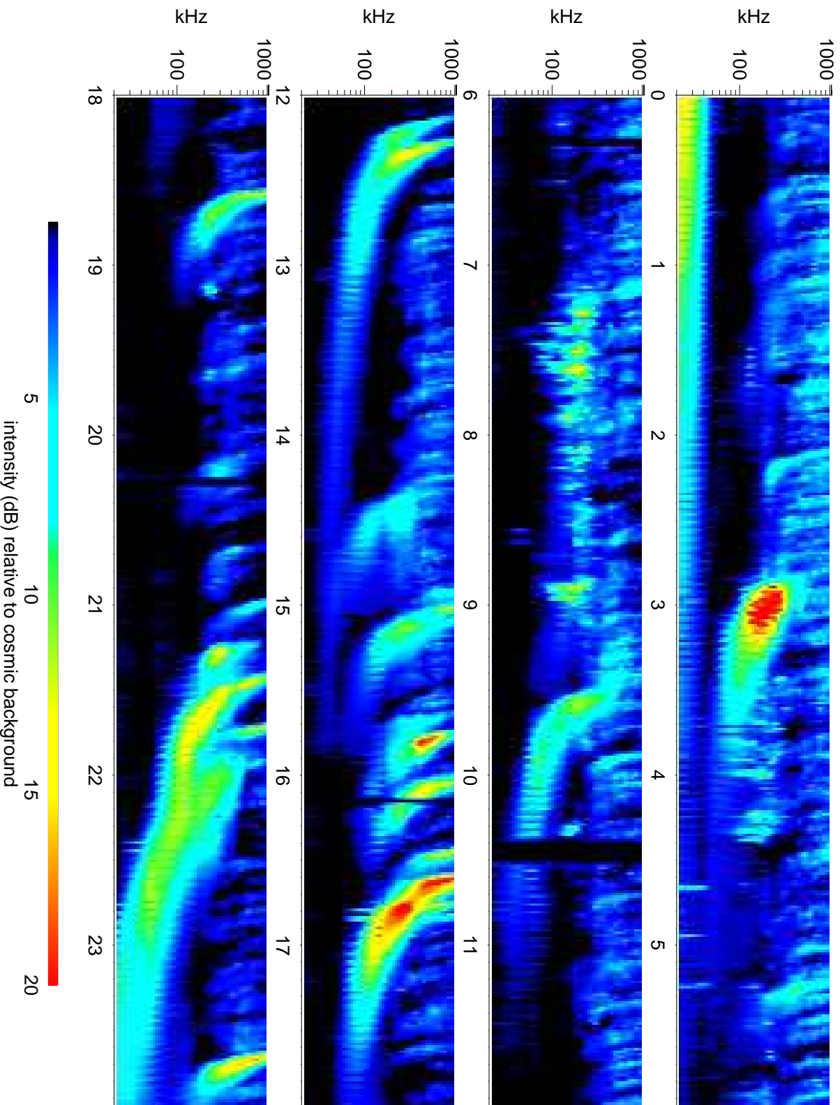
Wind Waves RAD1 receiver: 2011/08/01
