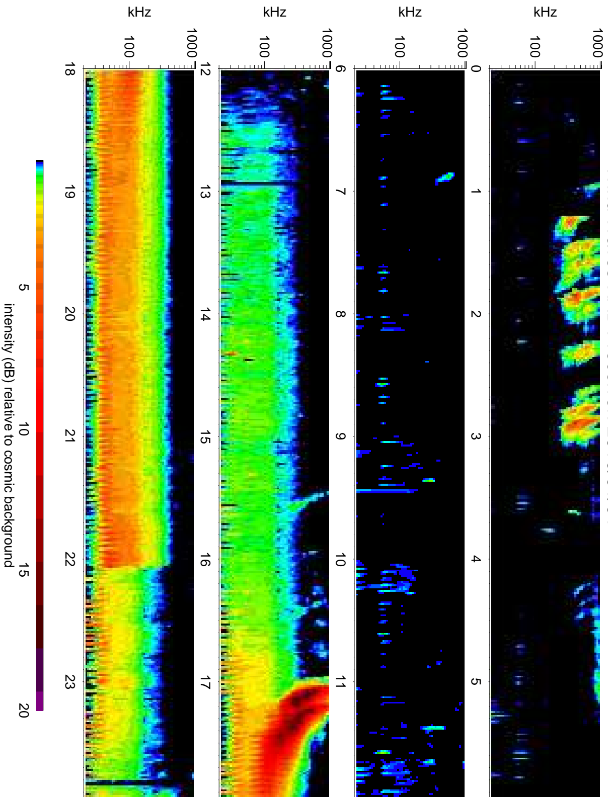
Wind Waves RAD1 receiver: 2010/01/01
