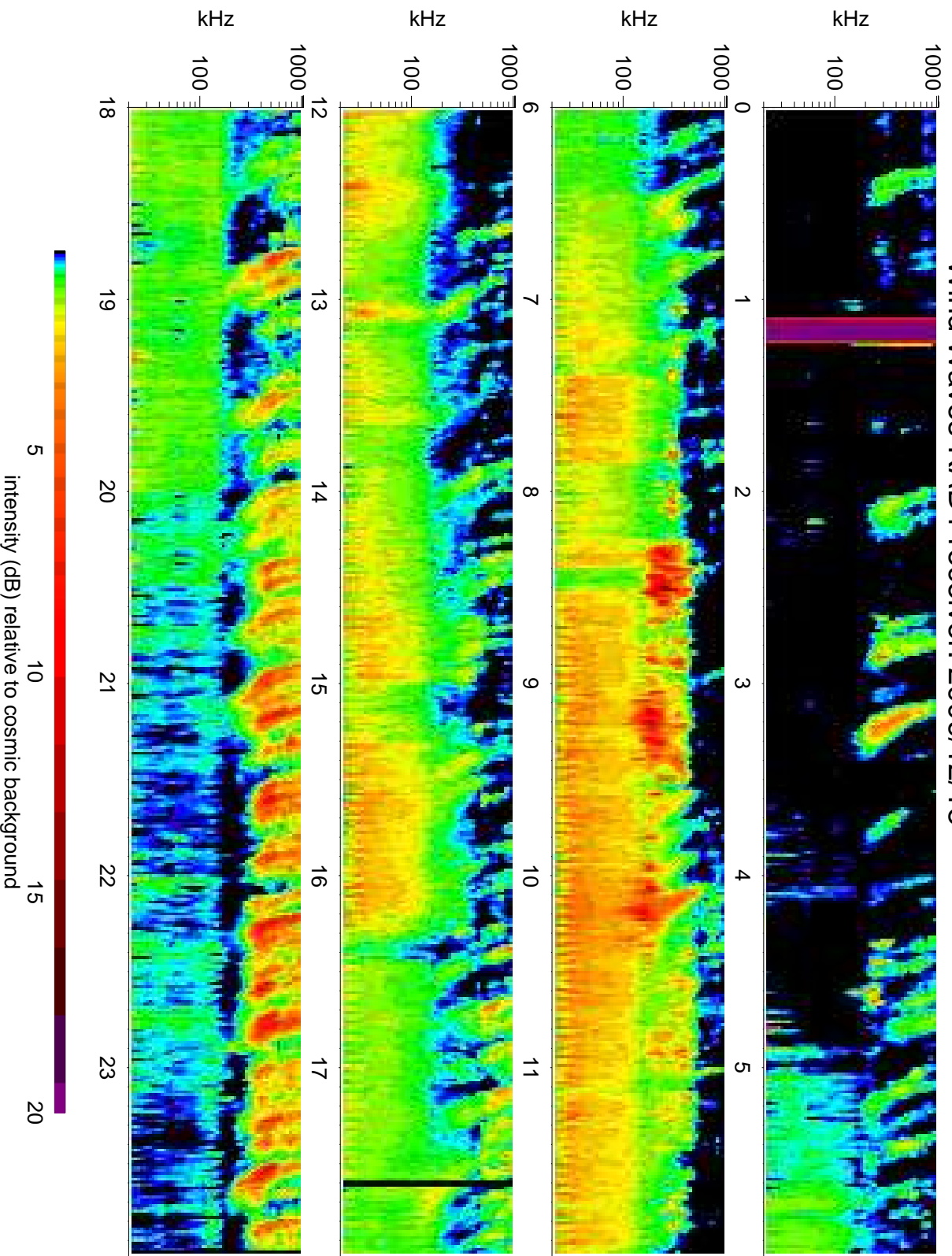
Wind Waves RAD1 receiver: 2009/12/18
