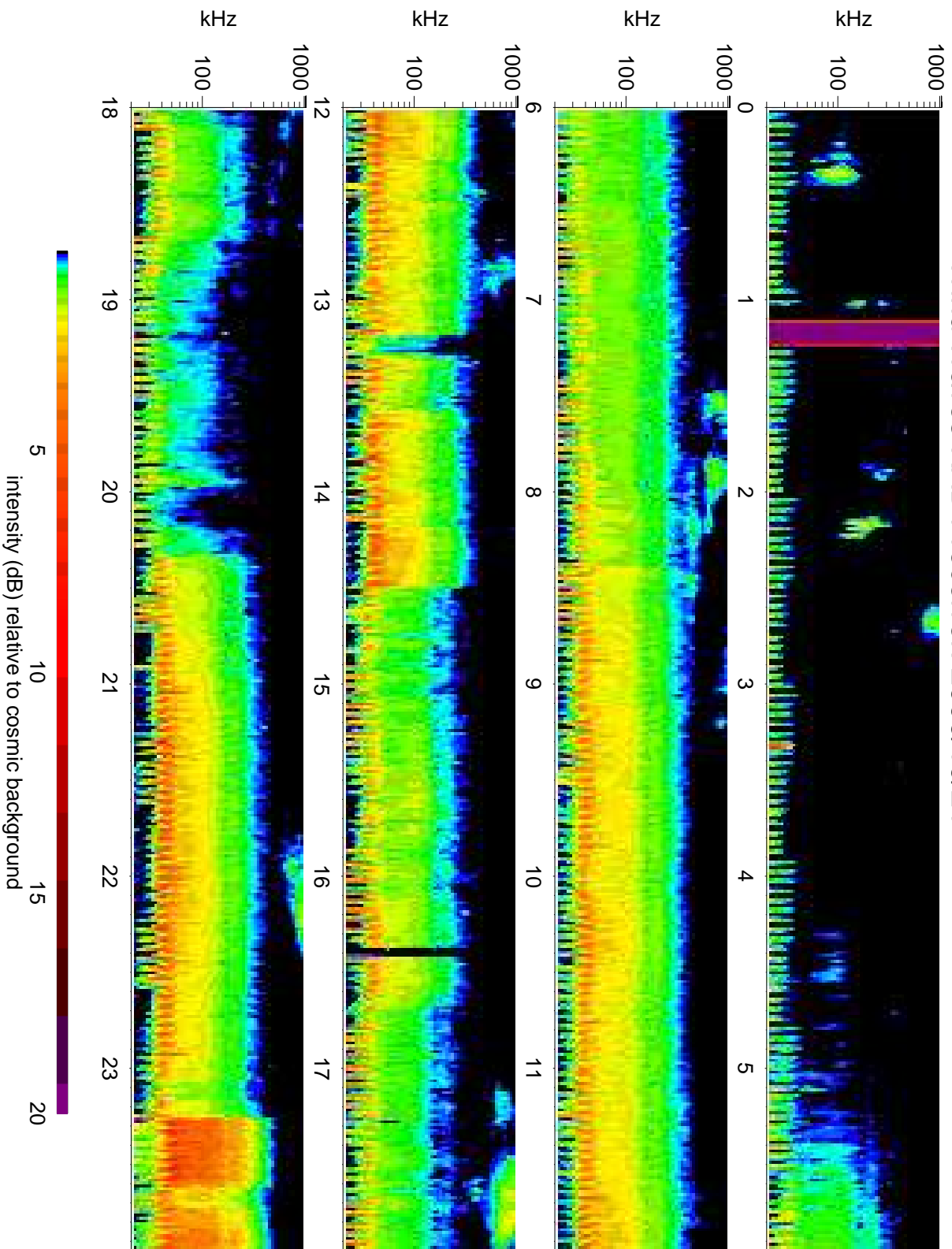
Wind Waves RAD1 receiver: 2009/10/21
