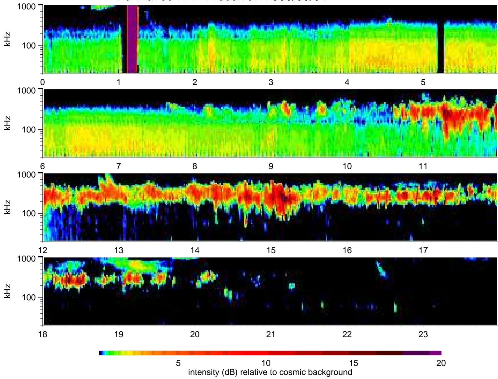
Wind Waves RAD1 receiver: 2009/05/04
