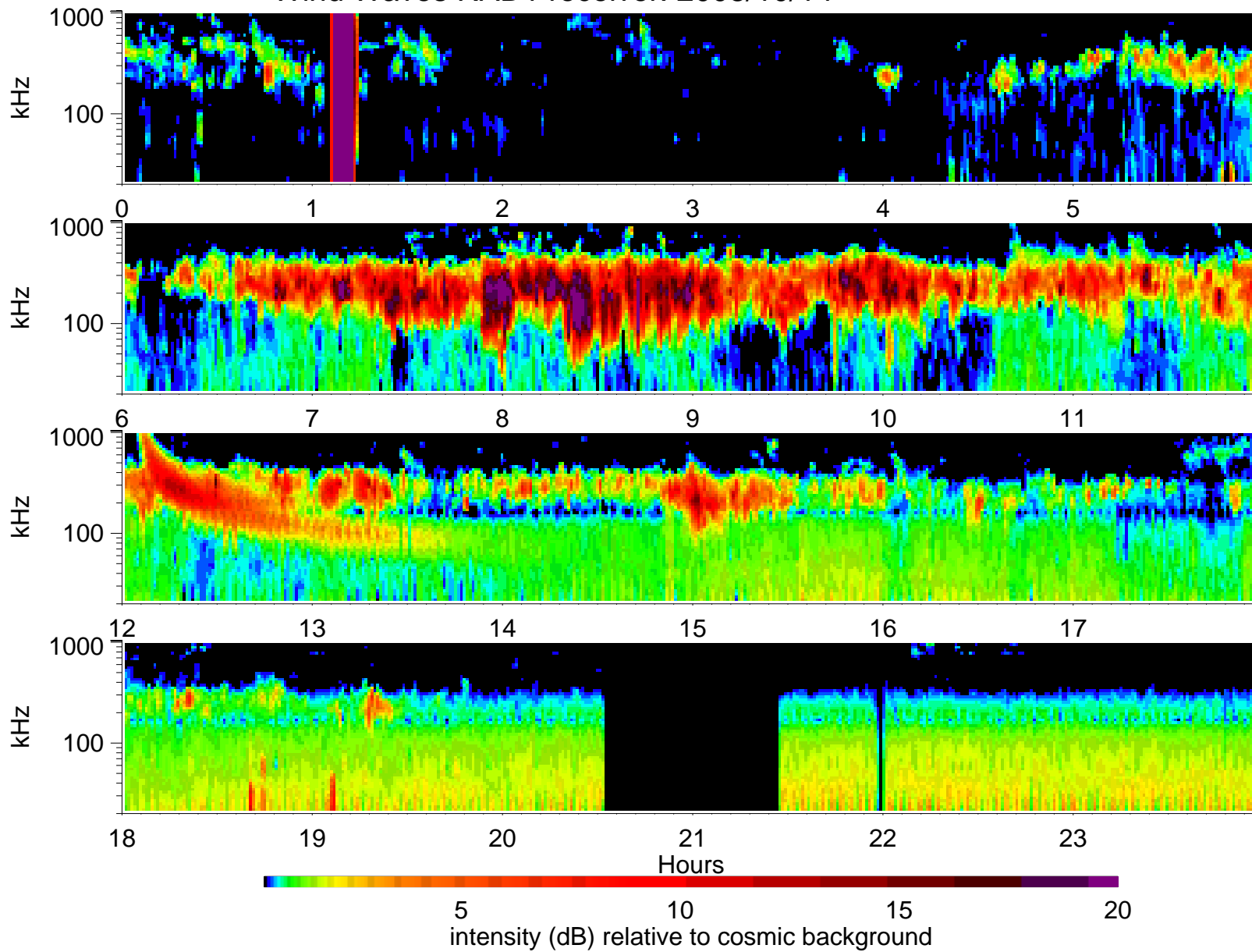
Wind Waves RAD1 receiver: 2008/10/14
