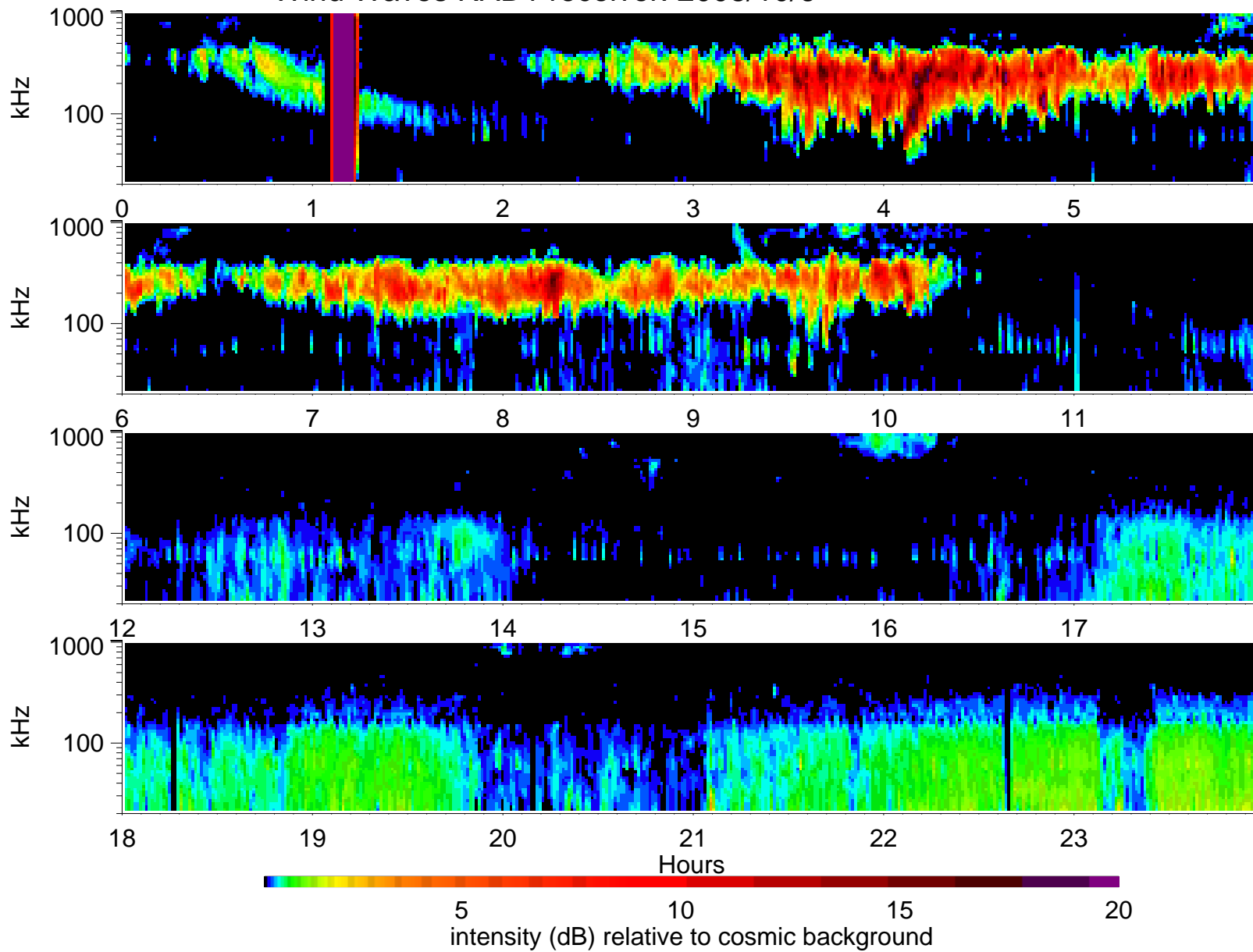
Wind Waves RAD1 receiver: 2008/10/6
