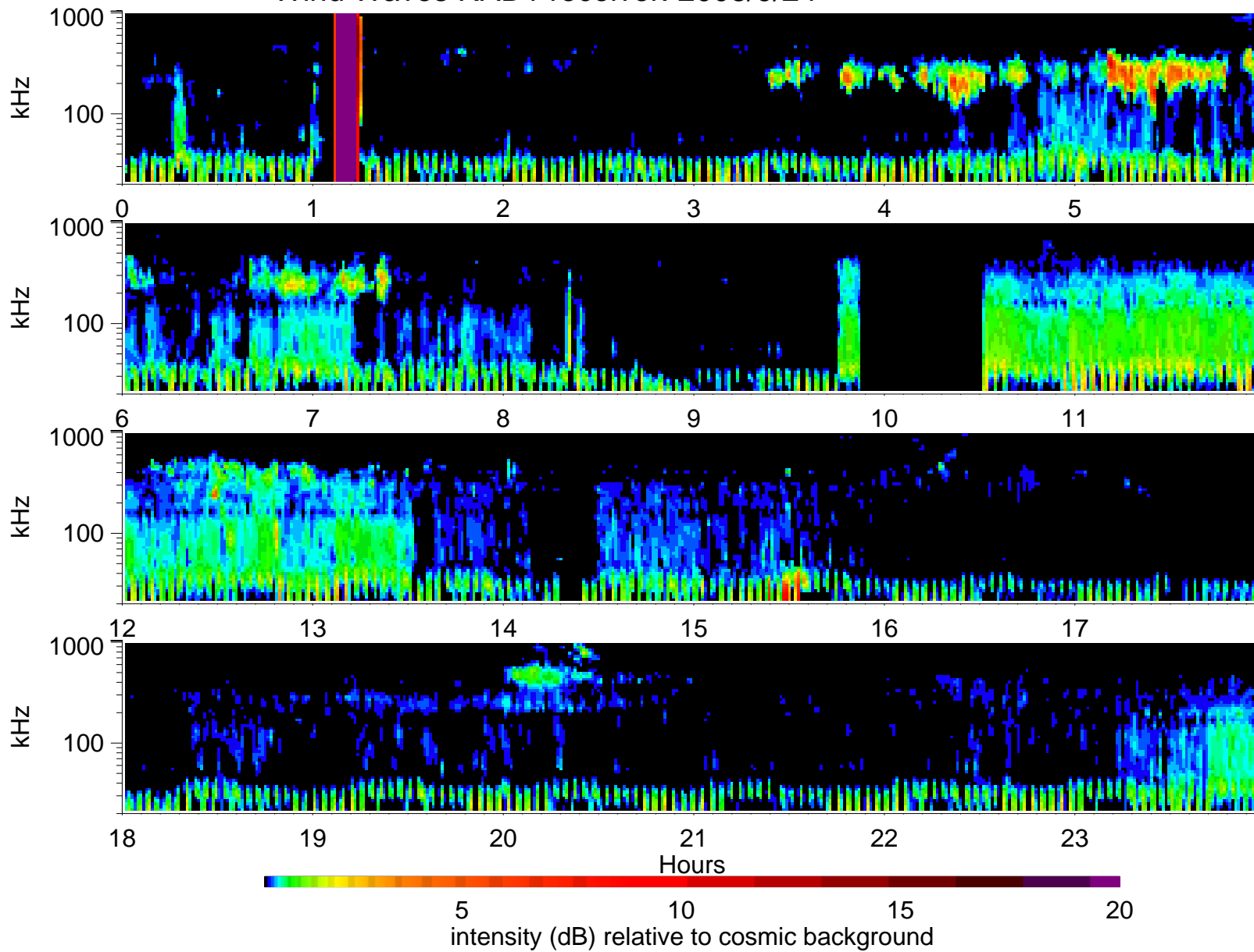
Wind Waves RAD1 receiver: 2008/9/24
