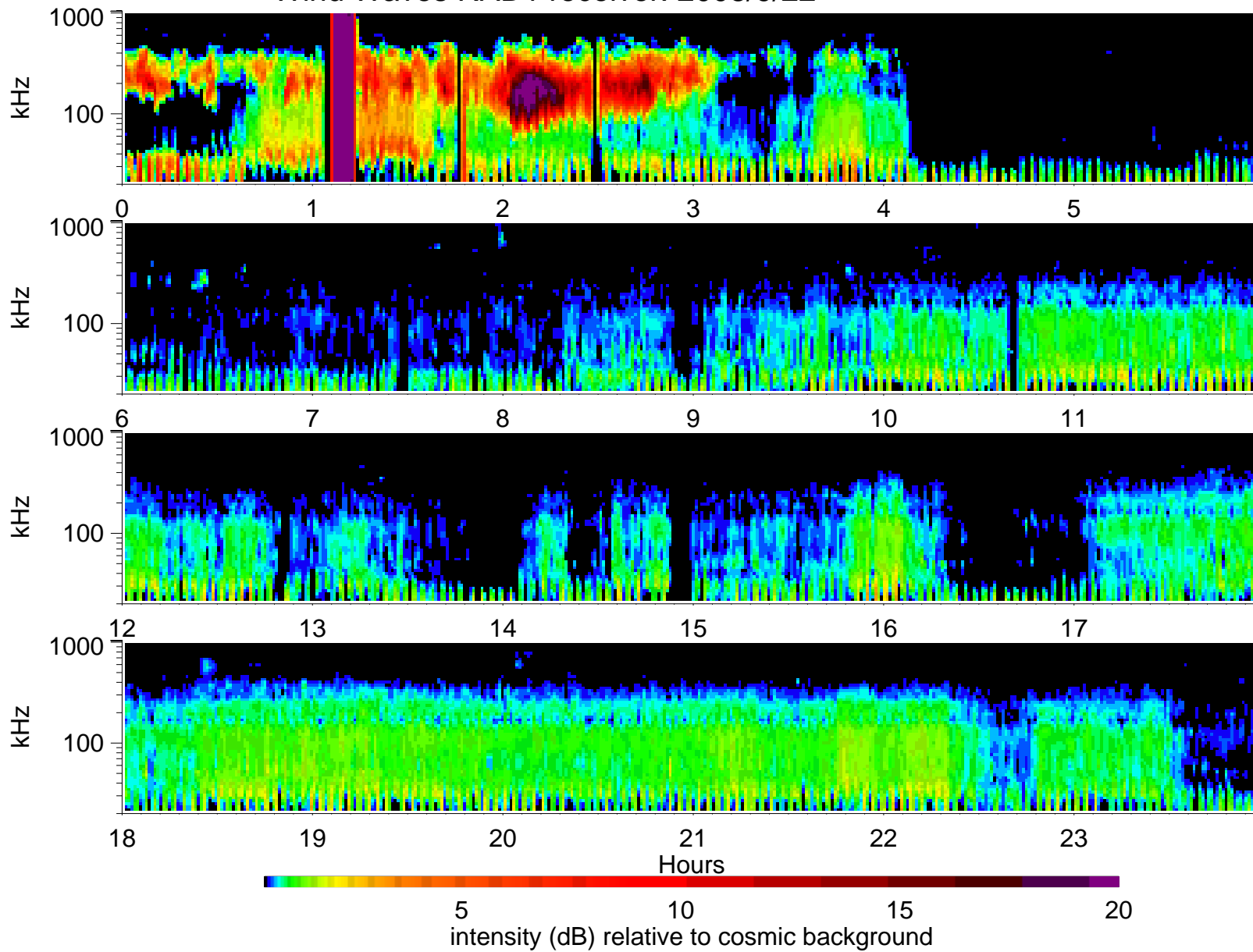
Wind Waves RAD1 receiver: 2008/9/22
