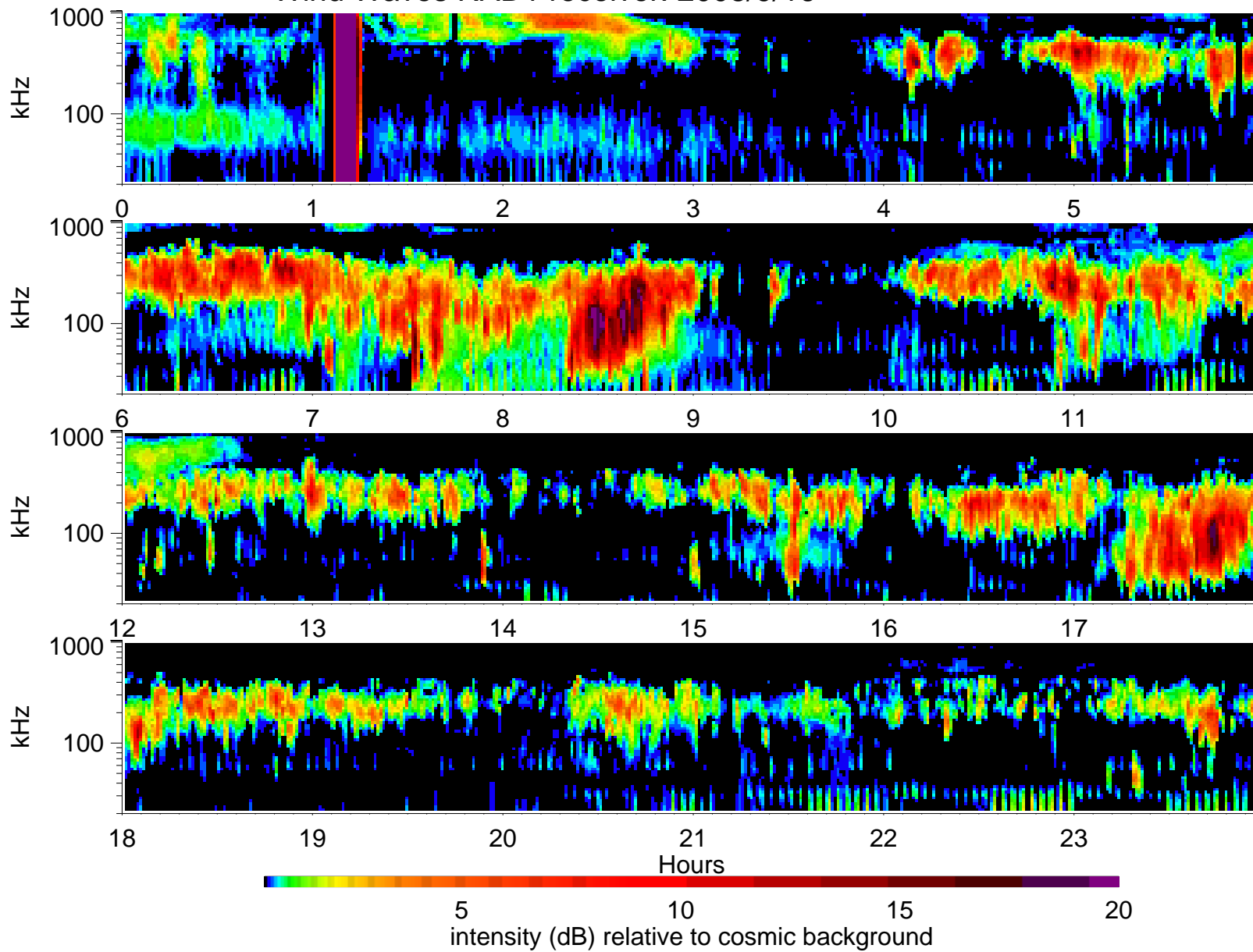
Wind Waves RAD1 receiver: 2008/9/16
