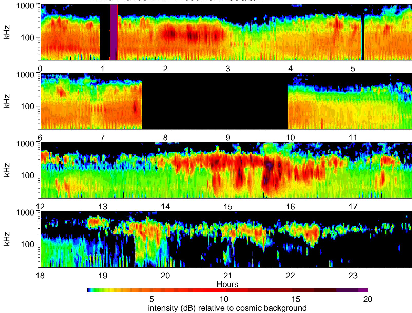
Wind Waves RAD1 receiver: 2008/9/4
