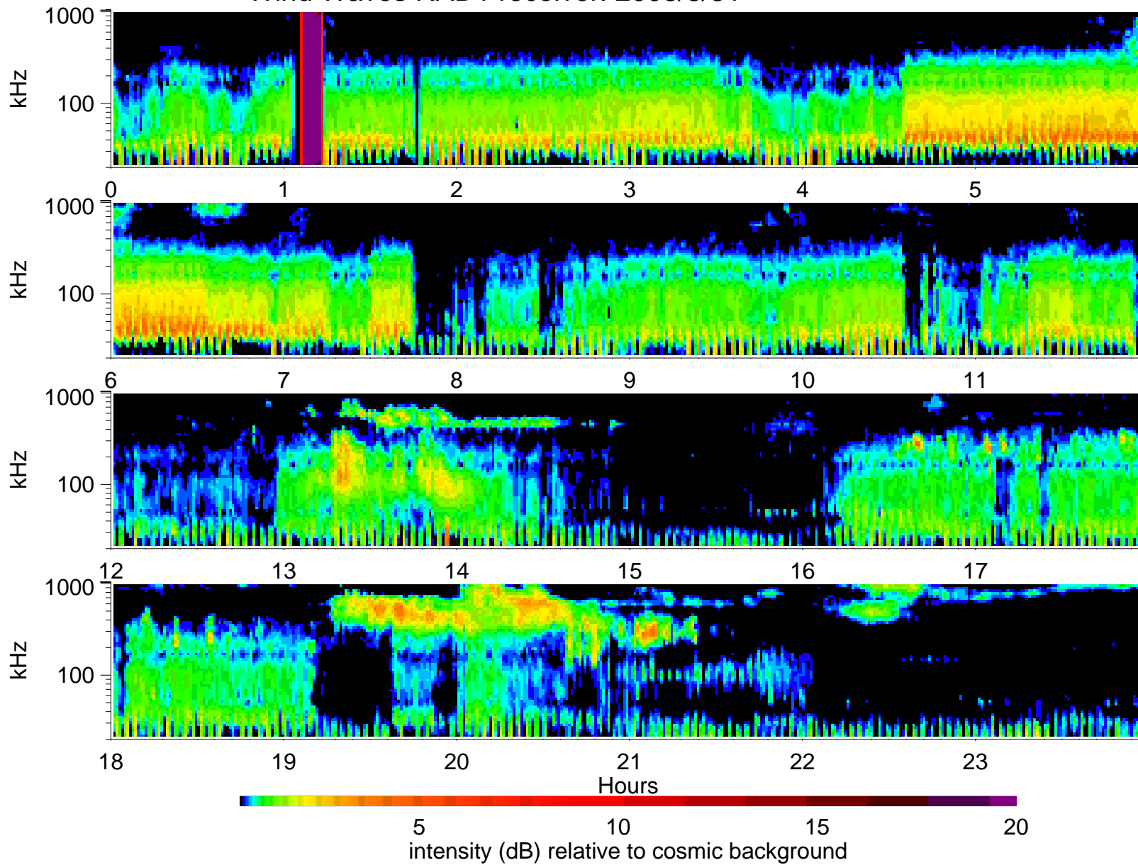
Wind Waves RAD1 receiver: 2008/8/31
