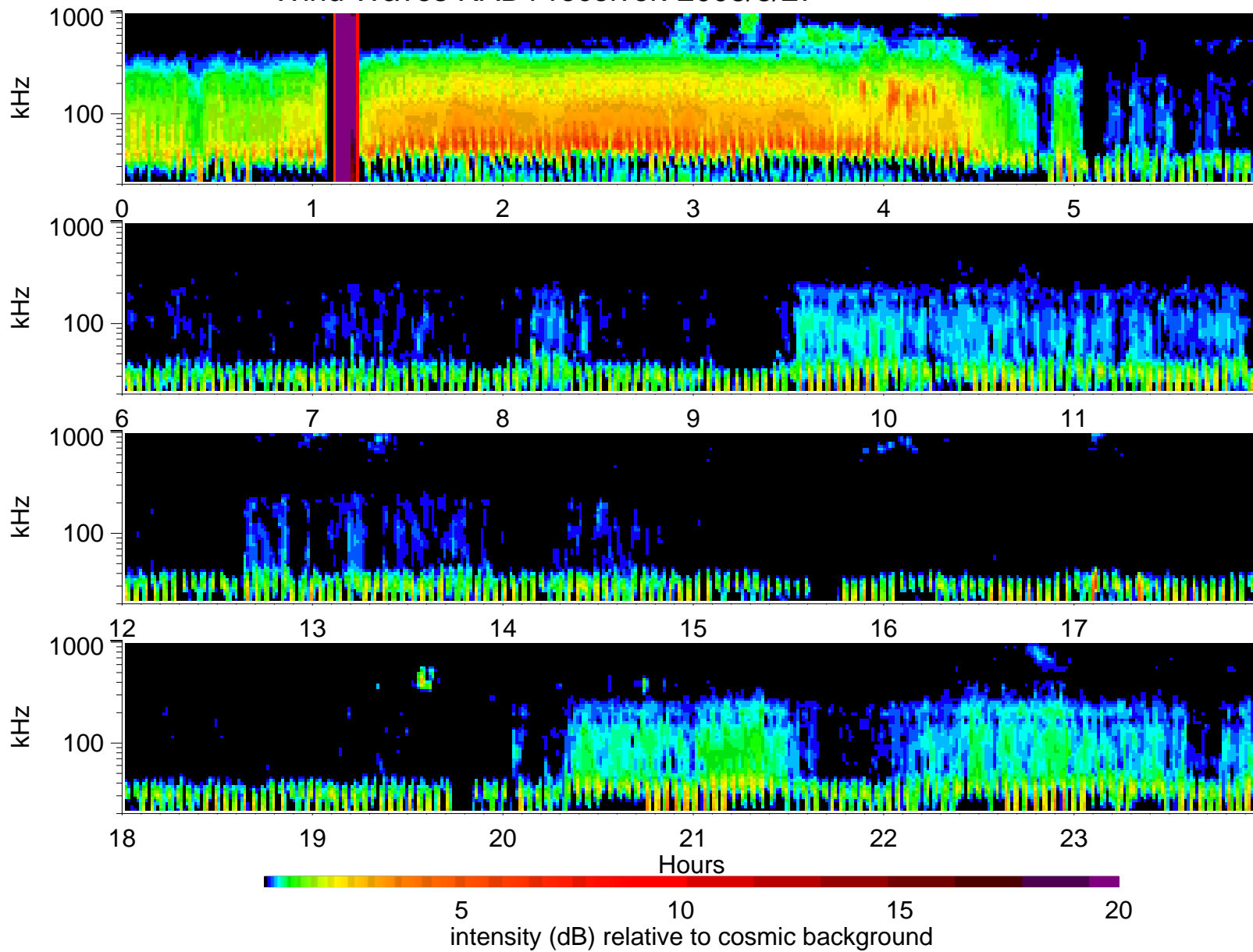
Wind Waves RAD1 receiver: 2008/8/27
