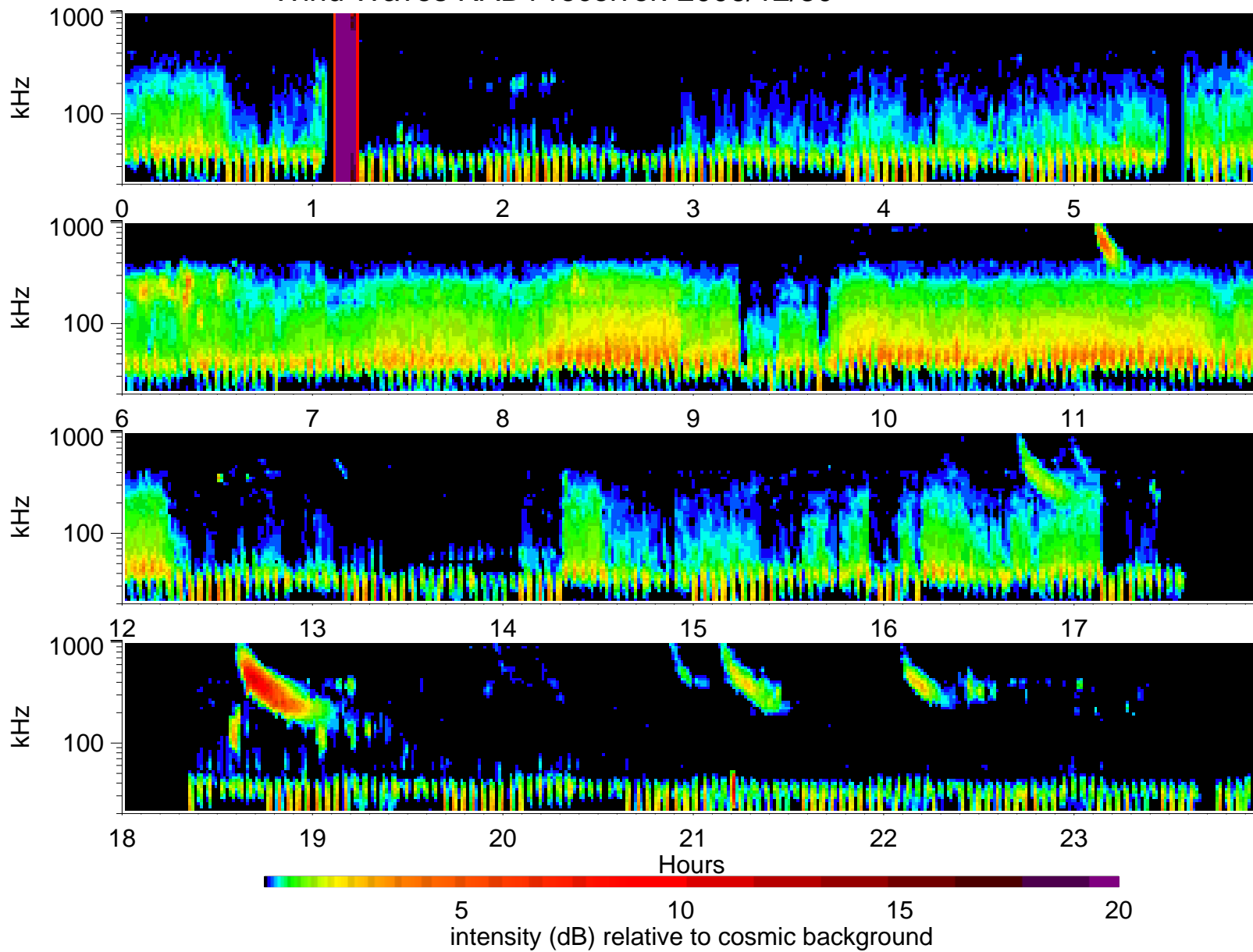
Wind Waves RAD1 receiver: 2006/12/30
