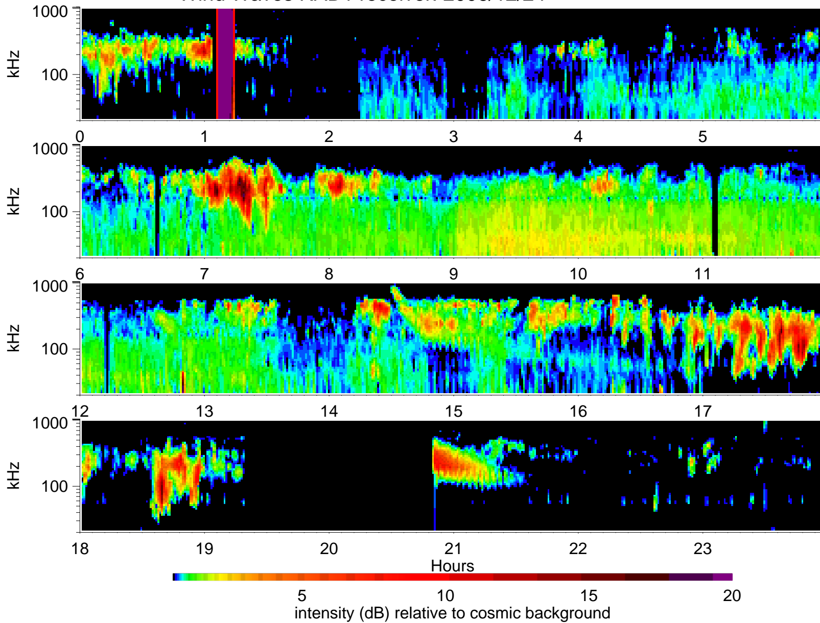
Wind Waves RAD1 receiver: 2006/12/24
