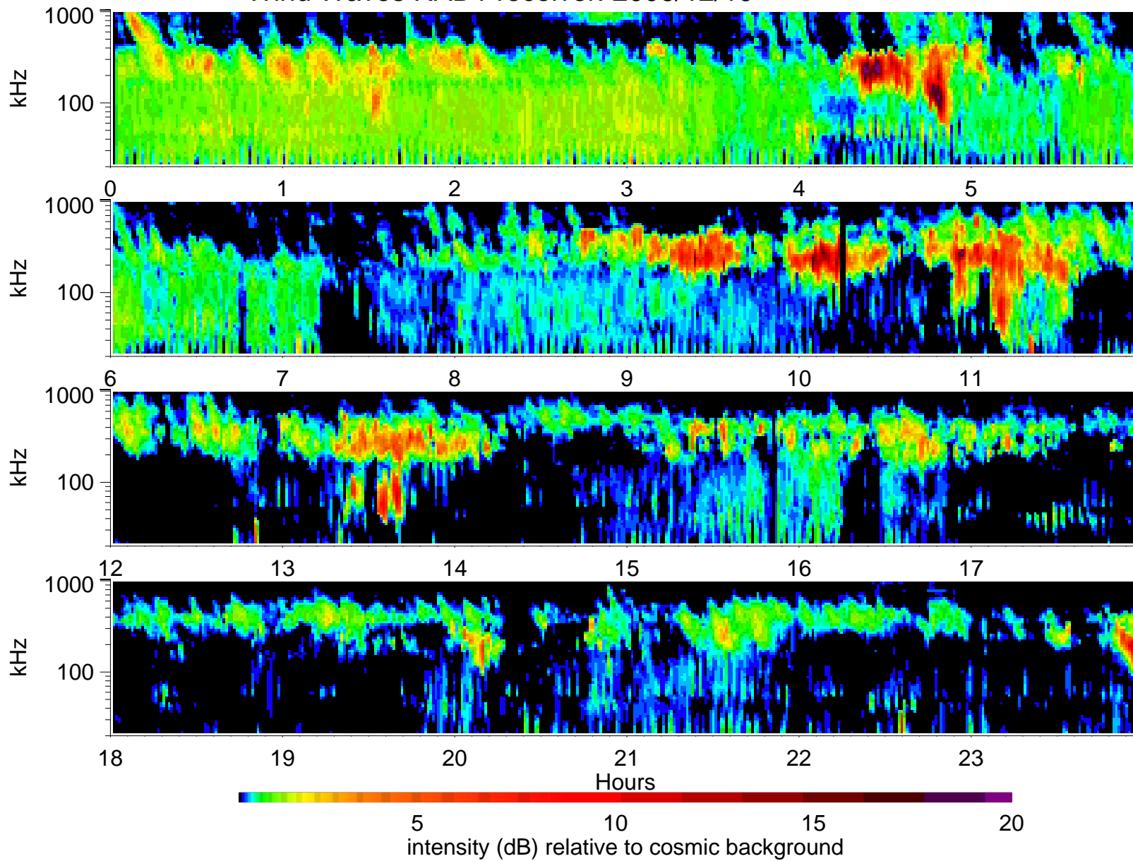
Wind Waves RAD1 receiver: 2006/12/19
