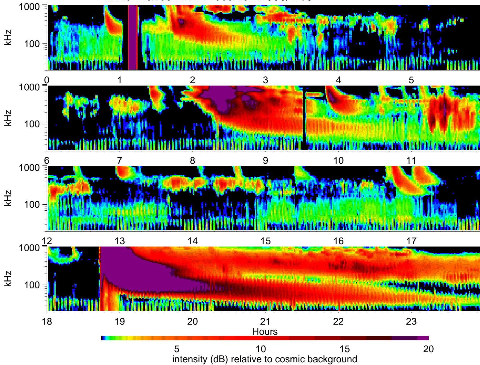
Wind Waves RAD1 receiver: 2006/12/6
