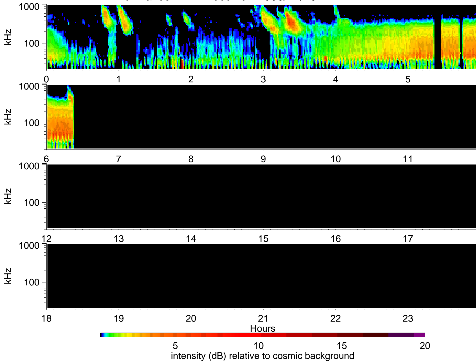
Wind Waves RAD1 receiver: 2006/11/23
