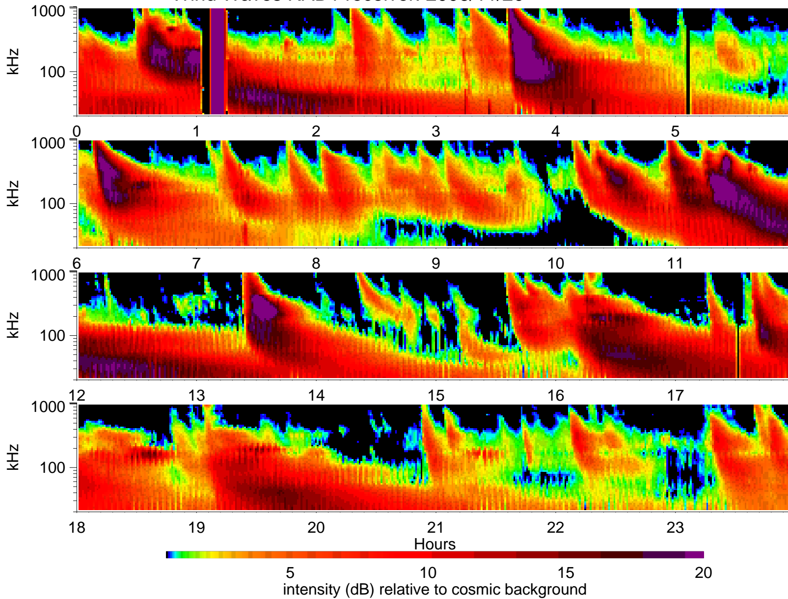
Wind Waves RAD1 receiver: 2006/11/20
