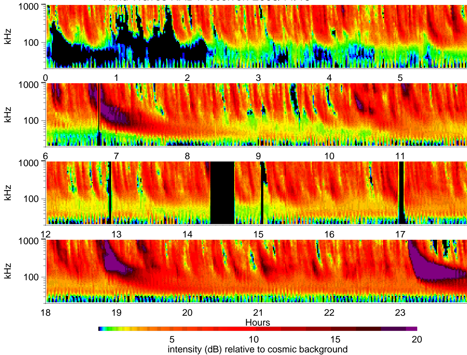
Wind Waves RAD1 receiver: 2006/11/15
