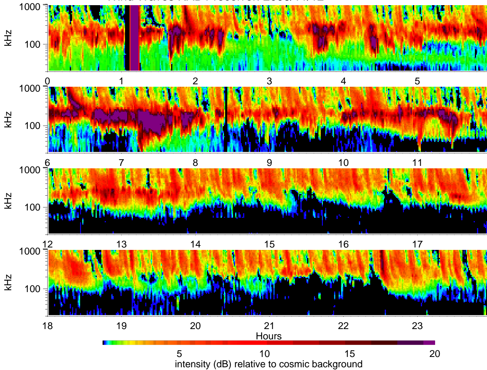
Wind Waves RAD1 receiver: 2006/11/12
