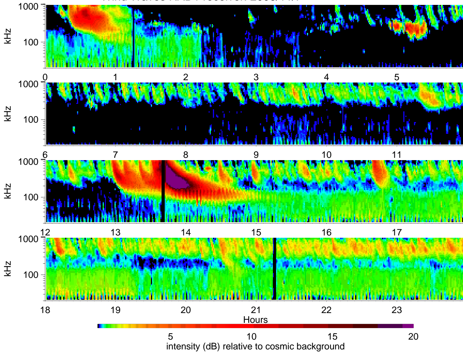
Wind Waves RAD1 receiver: 2006/11/7
