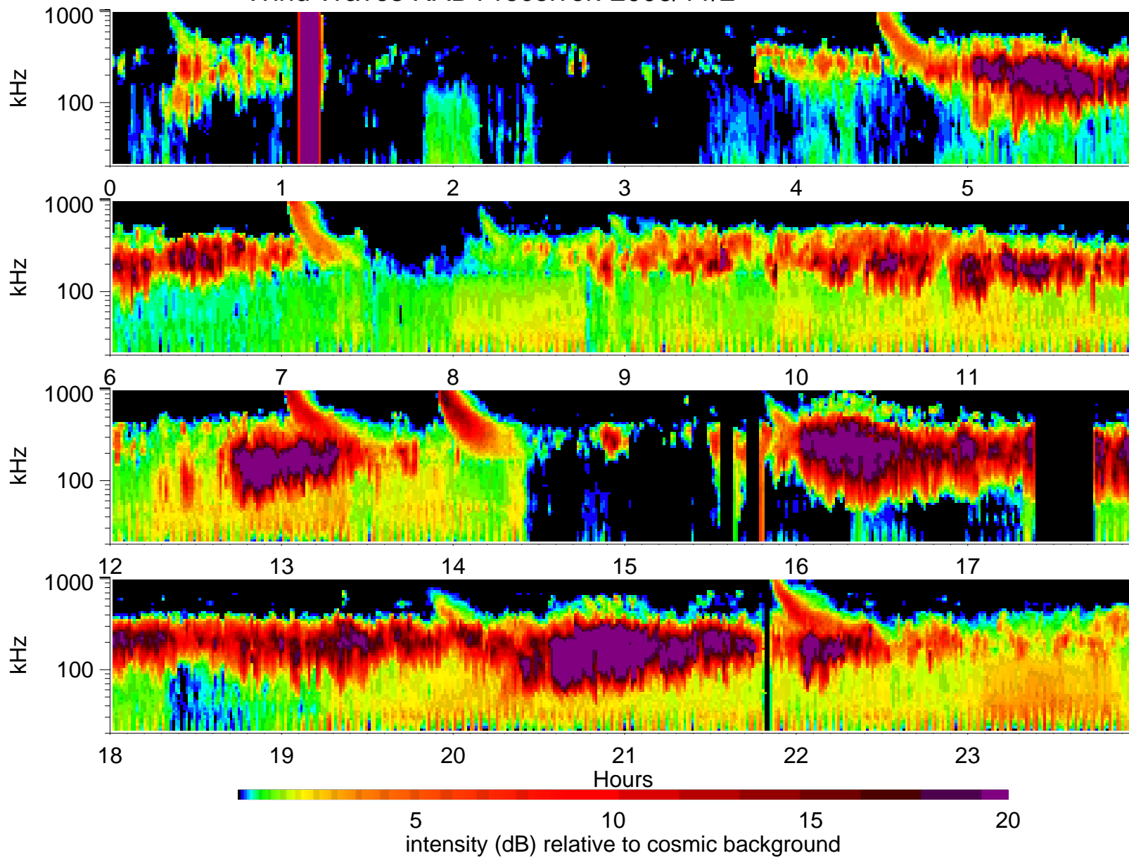
Wind Waves RAD1 receiver: 2006/11/2
