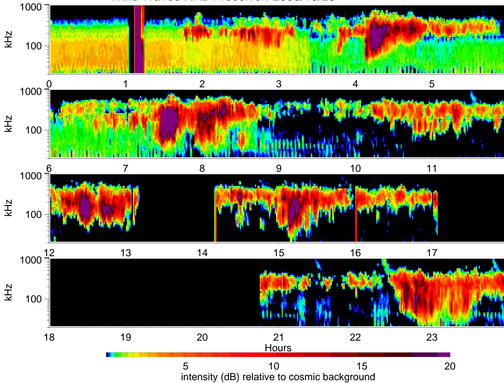
Wind Waves RAD1 receiver: 2006/10/29
