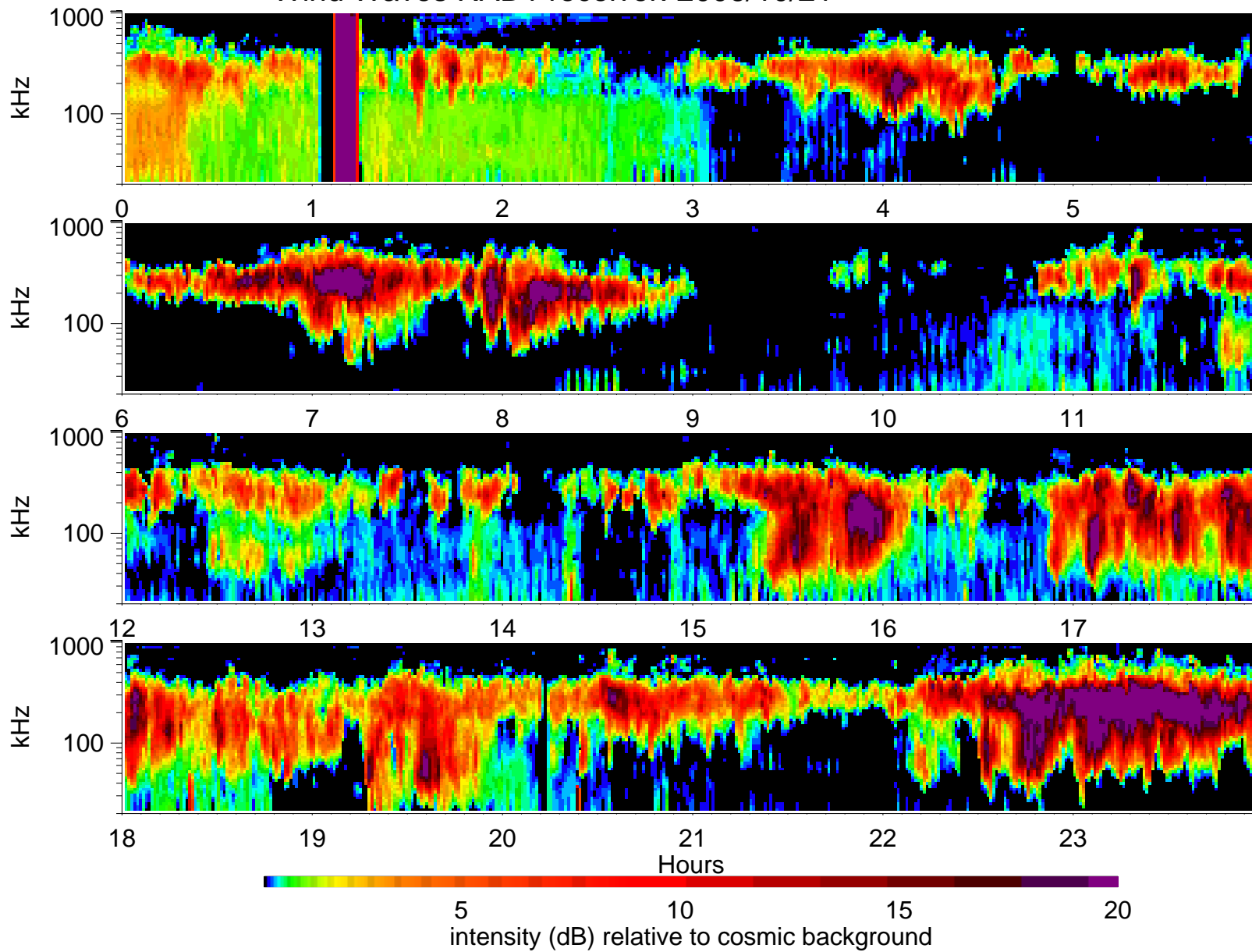
Wind Waves RAD1 receiver: 2006/10/21
