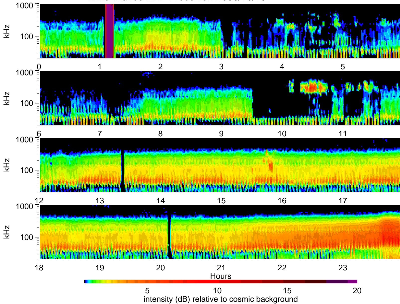
Wind Waves RAD1 receiver: 2006/10/19
