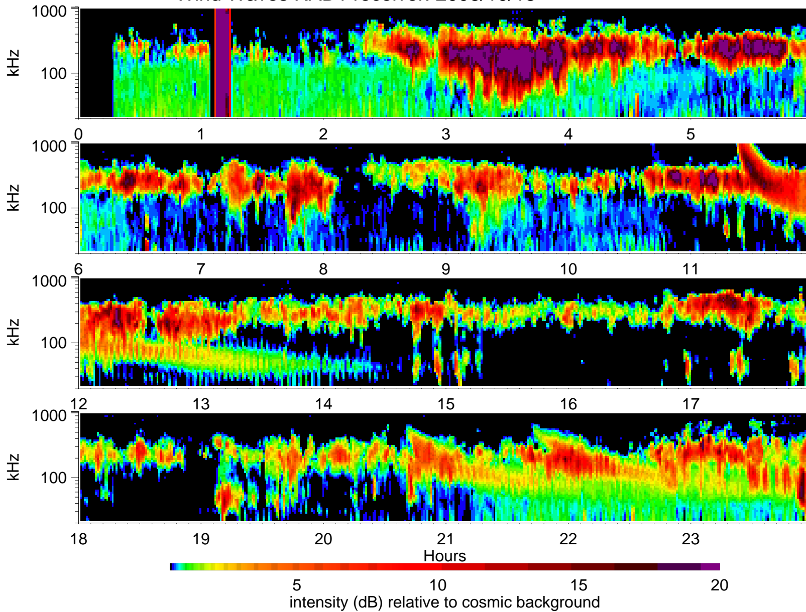
Wind Waves RAD1 receiver: 2006/10/15
