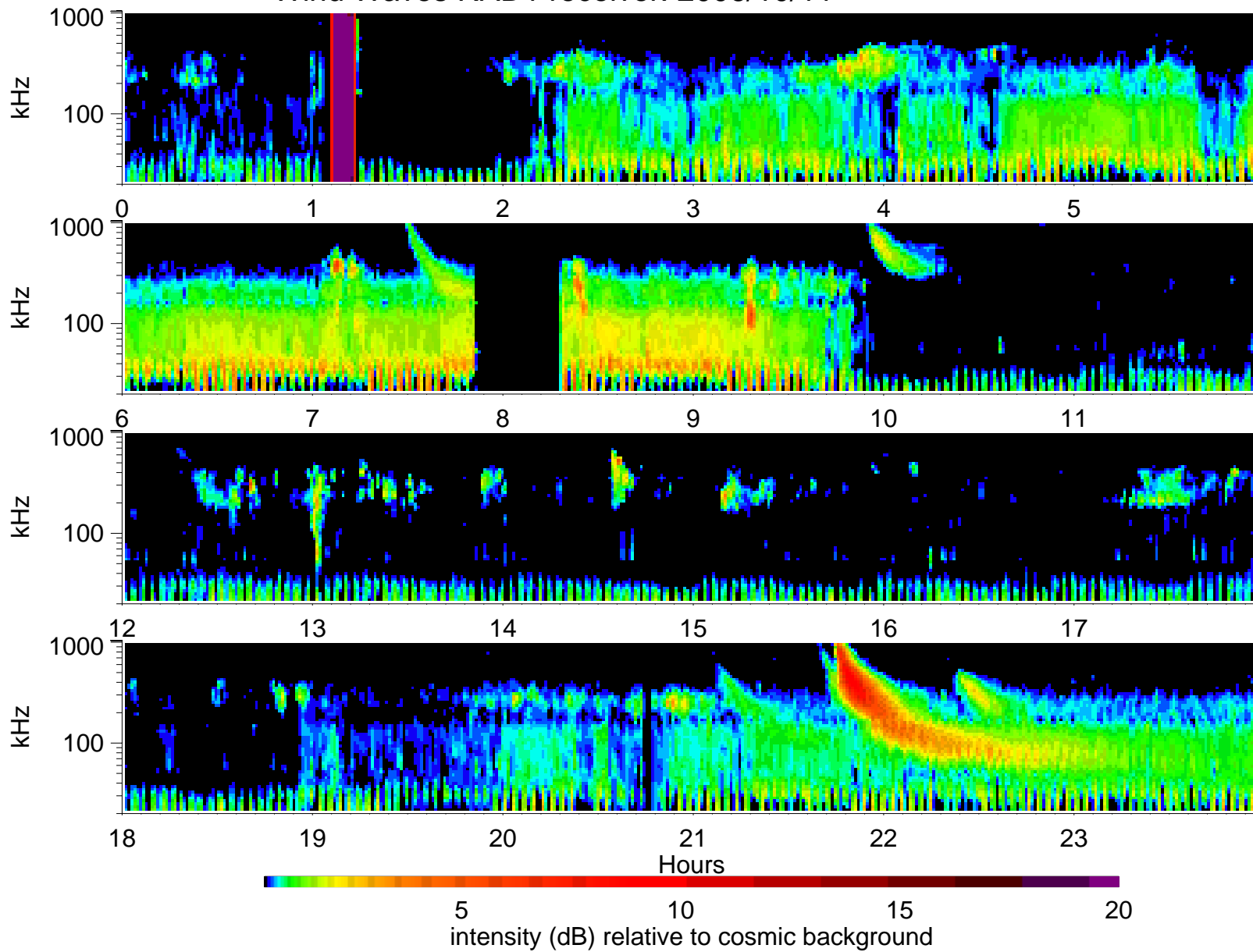
Wind Waves RAD1 receiver: 2006/10/11
