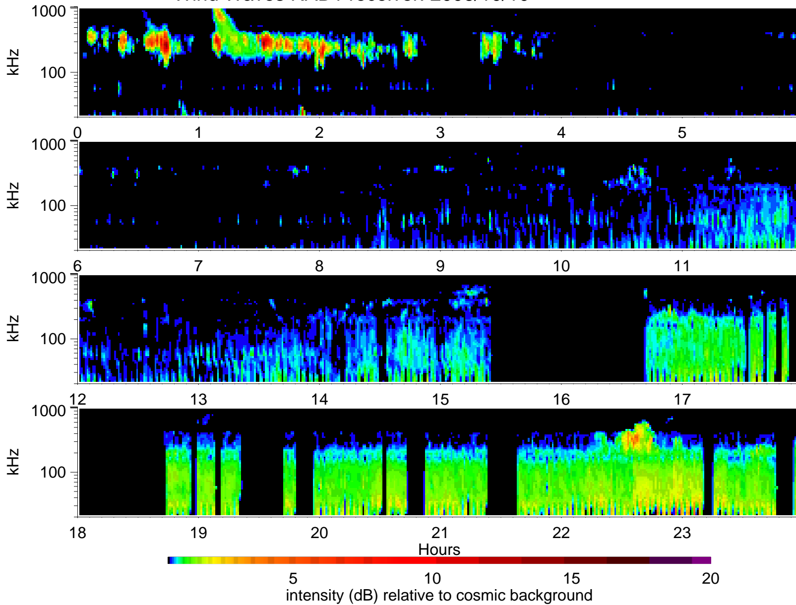
Wind Waves RAD1 receiver: 2006/10/10
