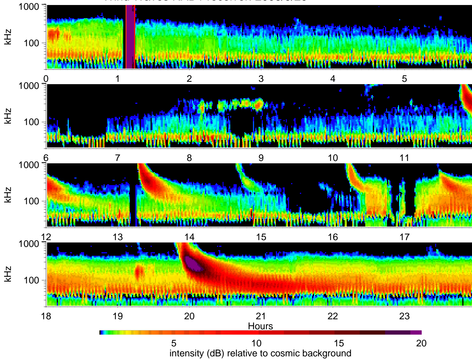
Wind Waves RAD1 receiver: 2006/9/29
