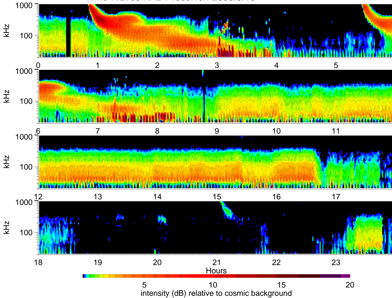
Wind Waves RAD1 receiver: 2006/9/16
