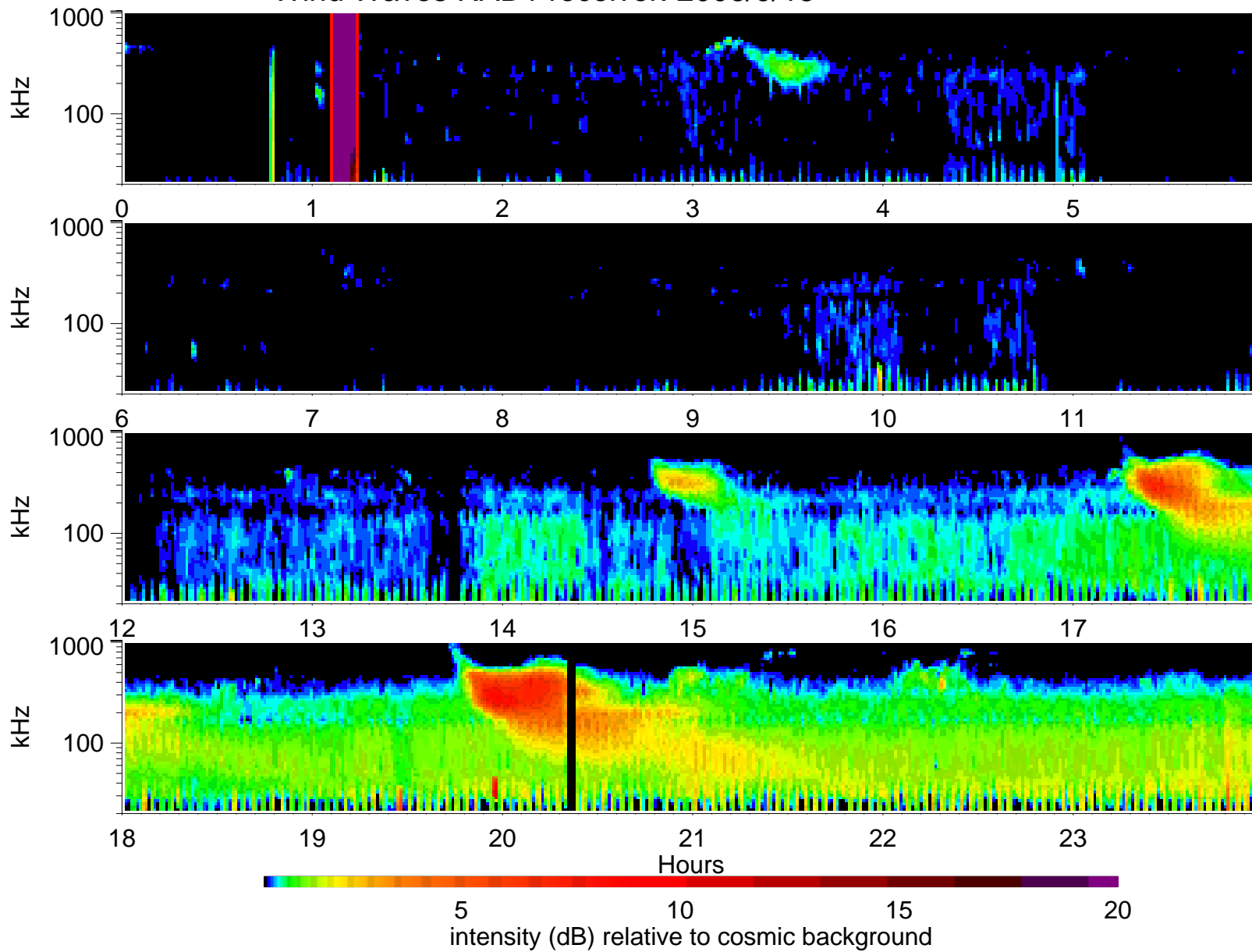
Wind Waves RAD1 receiver: 2006/9/15
