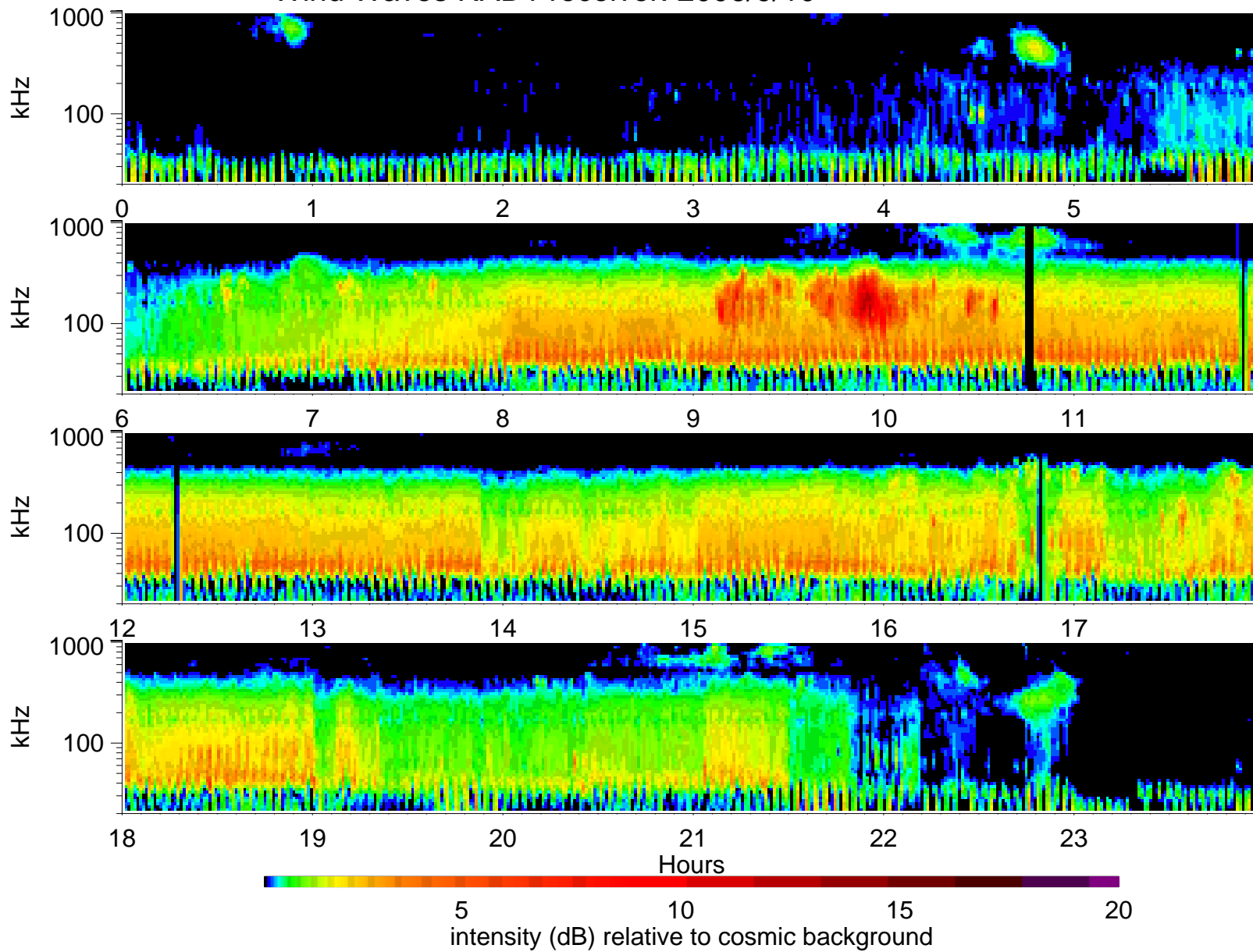
Wind Waves RAD1 receiver: 2006/9/10
