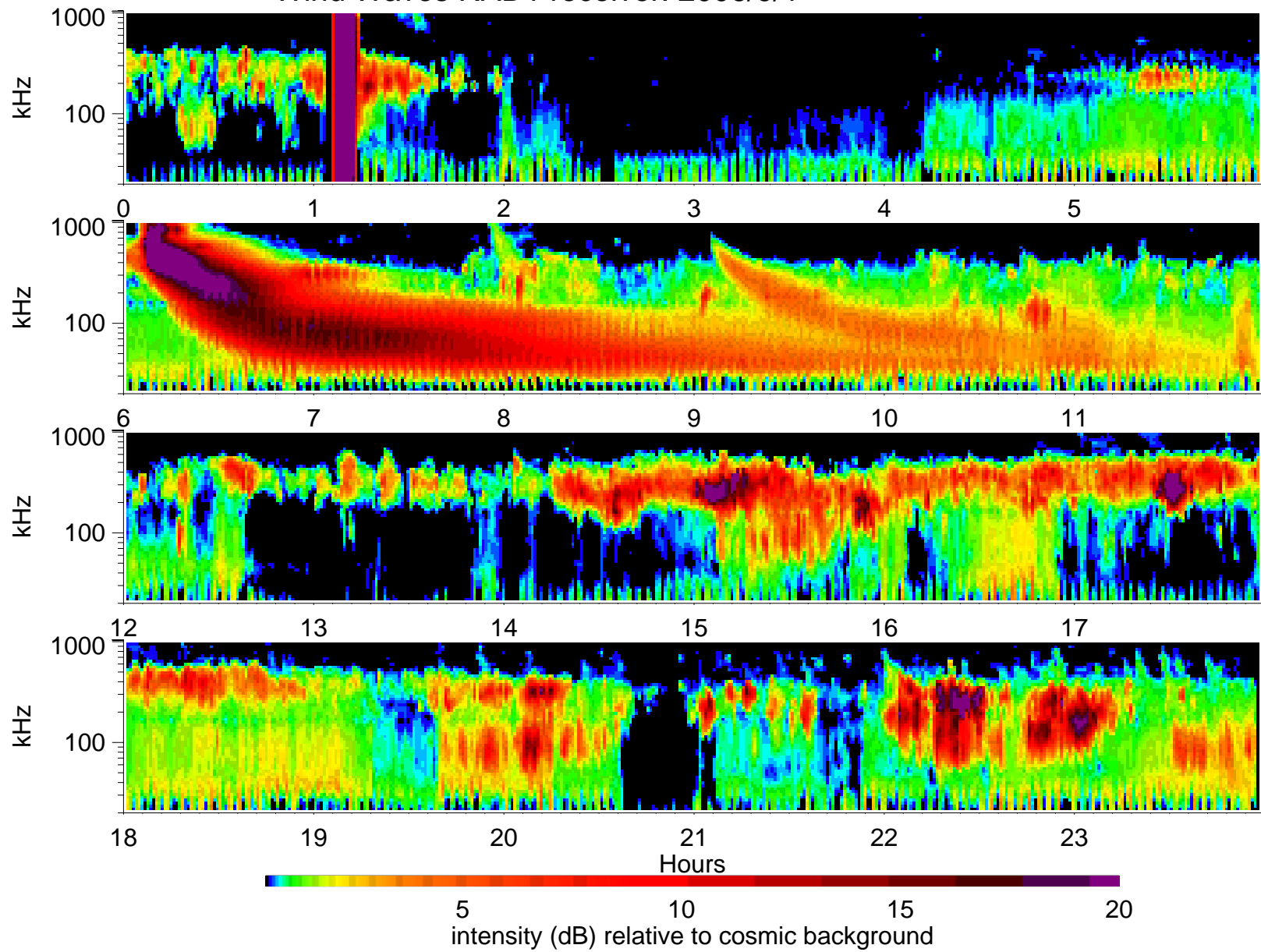
Wind Waves RAD1 receiver: 2006/9/1
