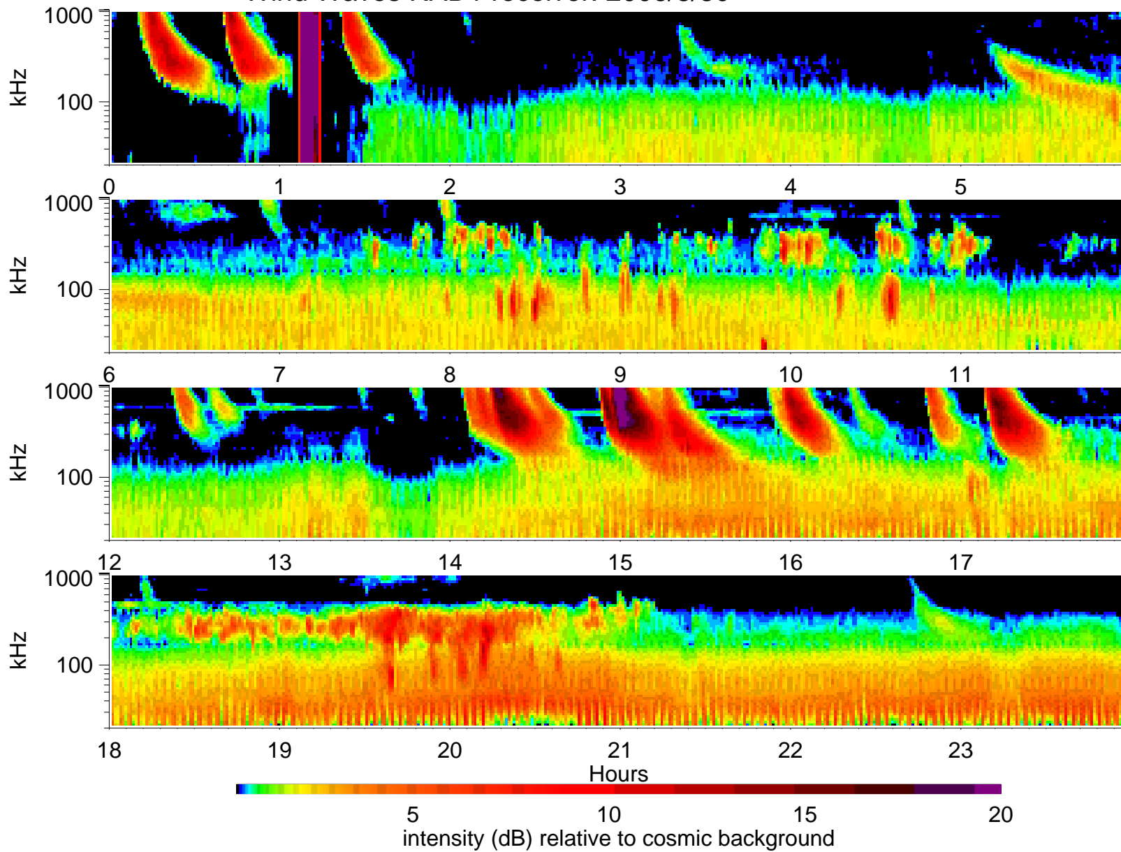
Wind Waves RAD1 receiver: 2006/8/30
