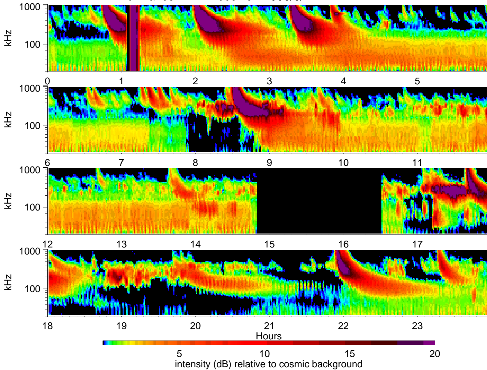
Wind Waves RAD1 receiver: 2006/8/22
