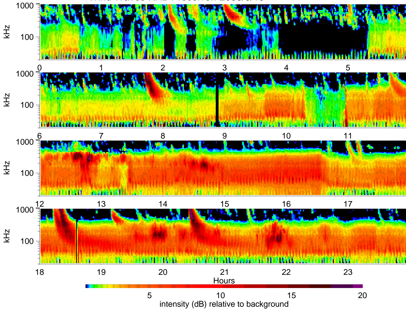
Wind Waves RAD1 receiver: 2006/8/19
