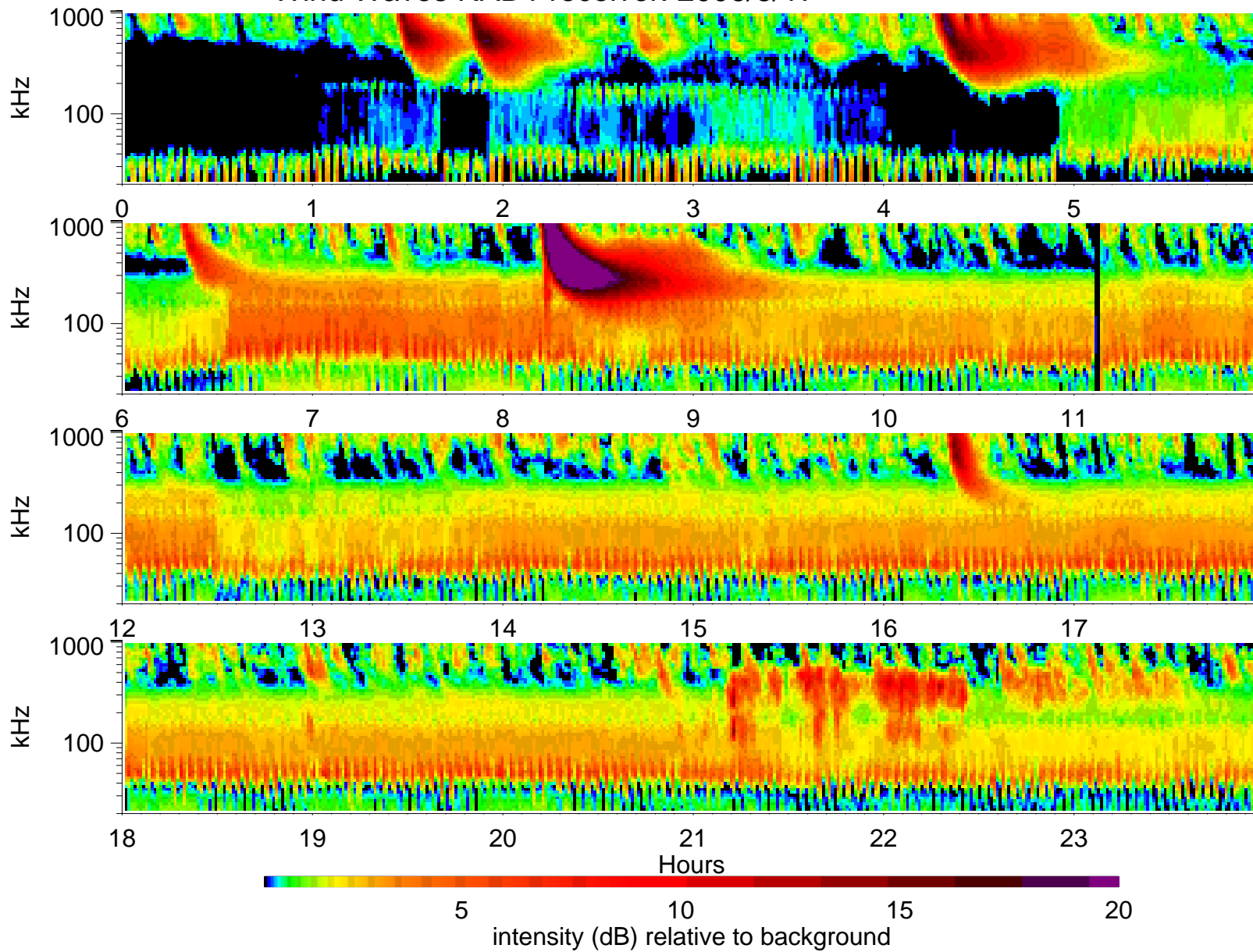
Wind Waves RAD1 receiver: 2006/8/17
