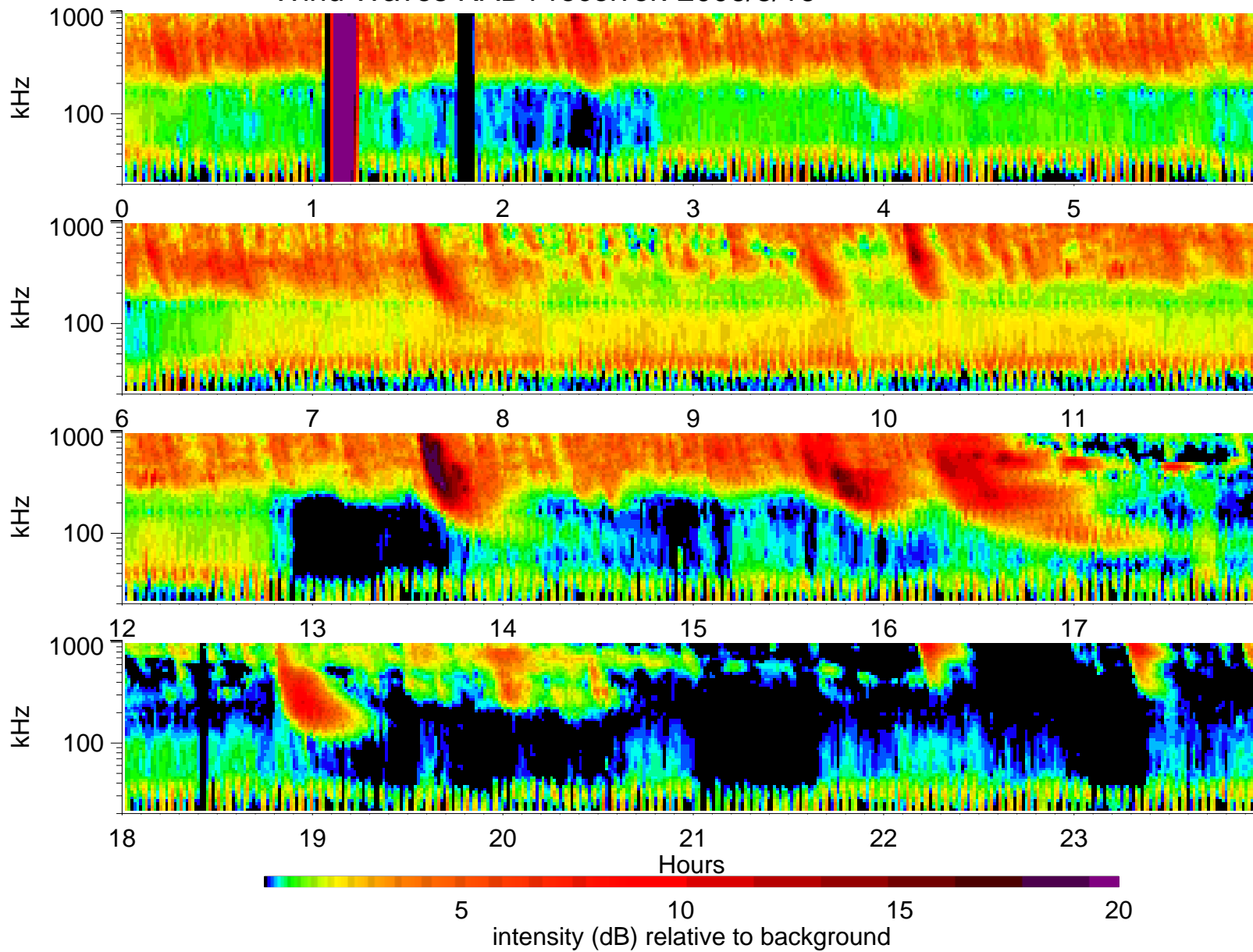
Wind Waves RAD1 receiver: 2006/8/16
