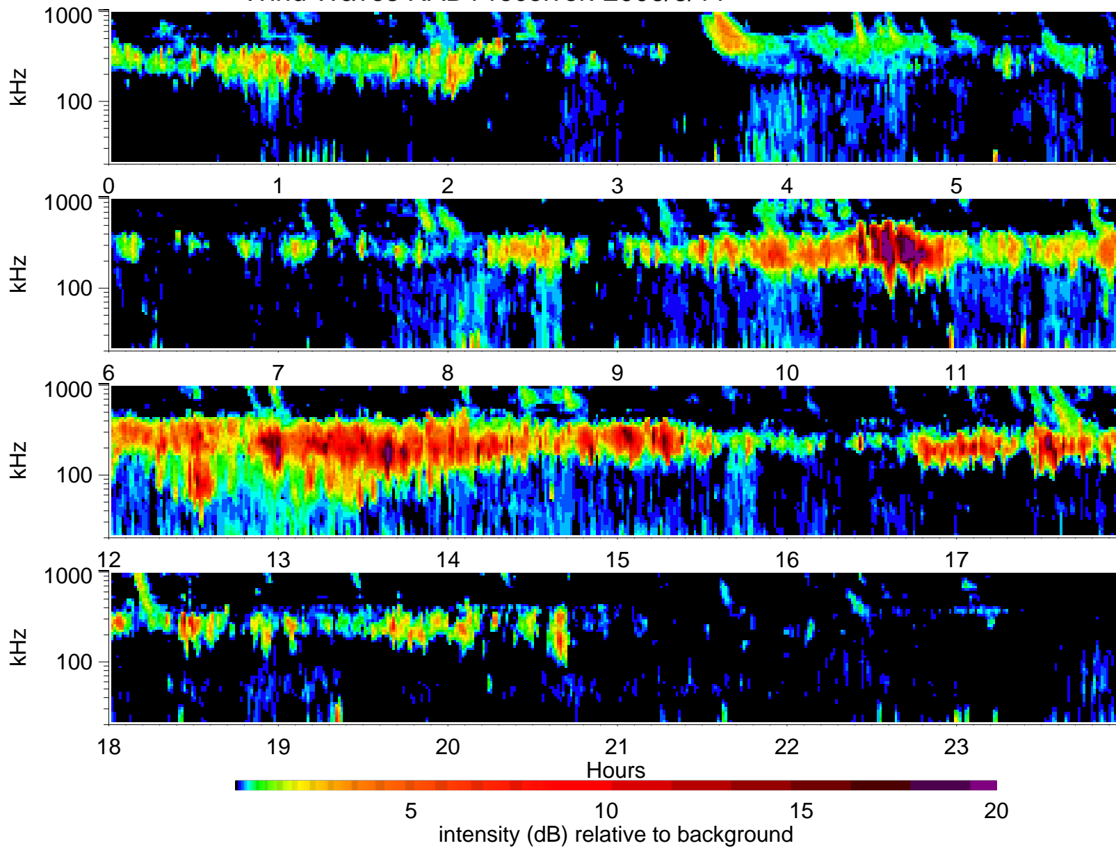
Wind Waves RAD1 receiver: 2006/8/11
