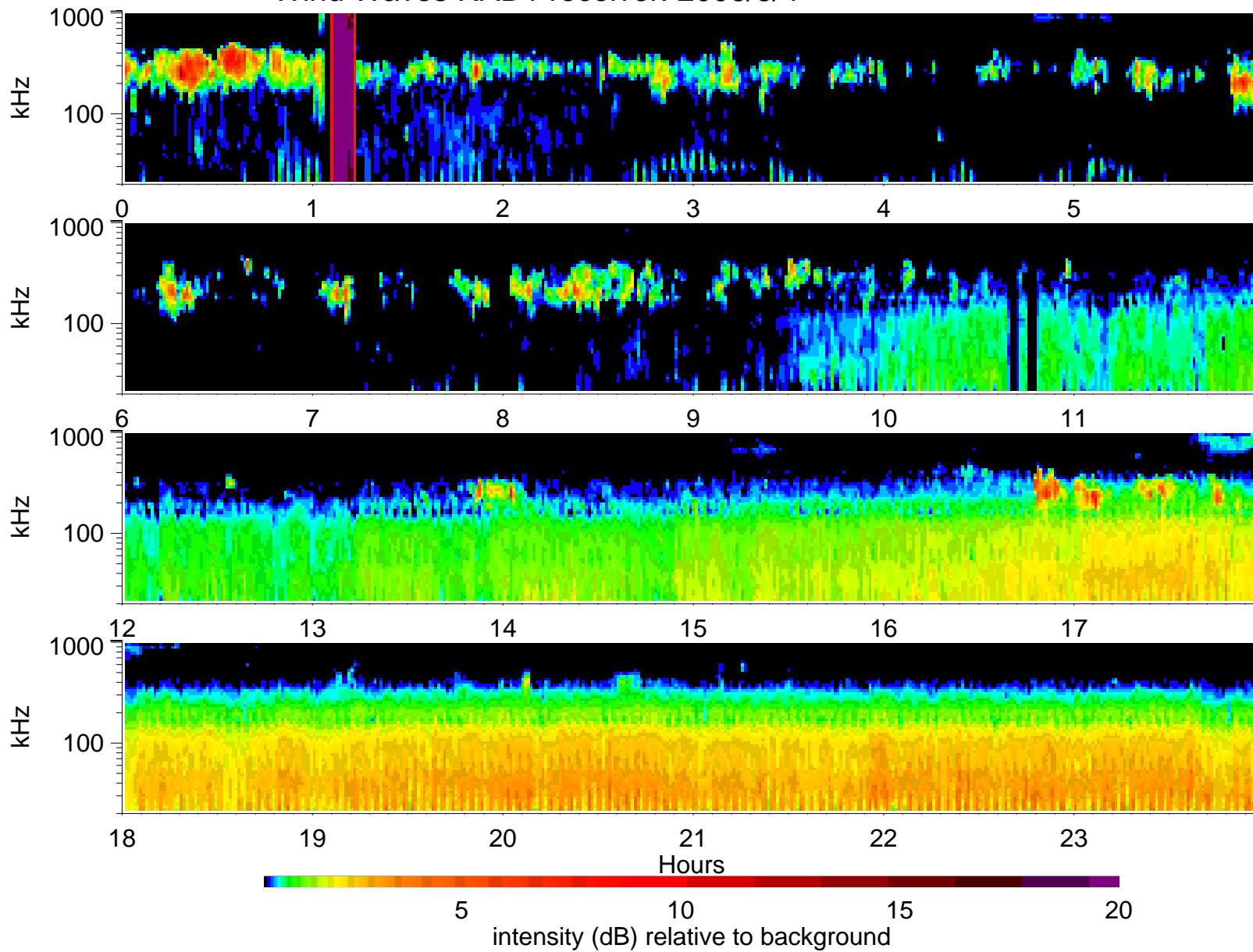
Wind Waves RAD1 receiver: 2006/8/4
