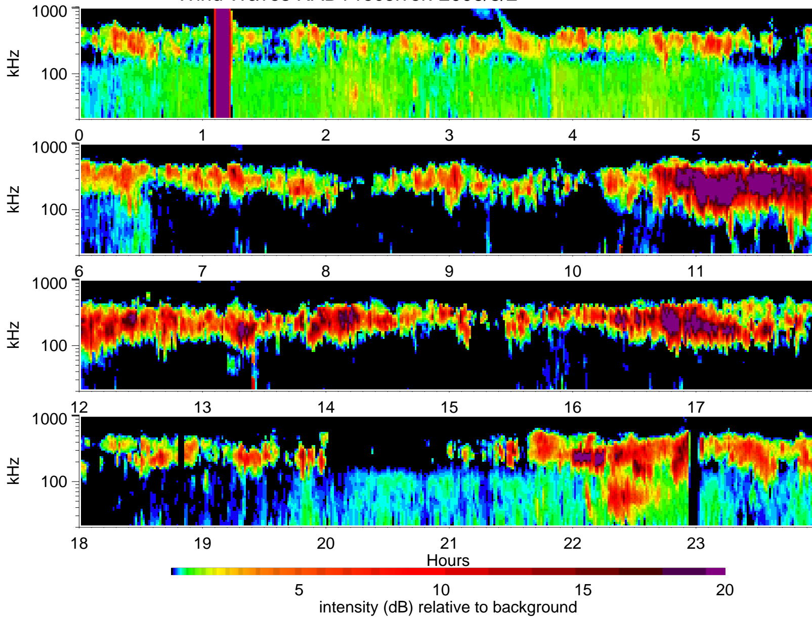
Wind Waves RAD1 receiver: 2006/8/2
